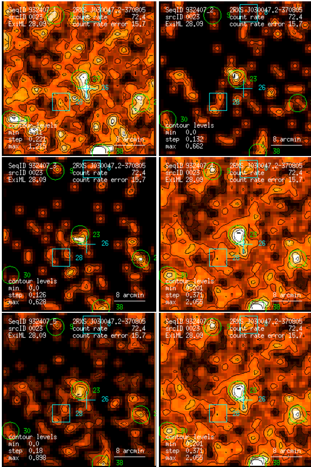
Figure 23: RASS 932407: detection 0023: band rate images, Gaussian filter: (1) PSPC channels 11 – 41, (2) 52 – 90, (3) 91 – 201, (4) 11 – 235, (5) 52 – 201, (6) 11 – 201. Broad band rates in counts/ks. Band rate contour levels in counts/ks/arcmin 2 .
