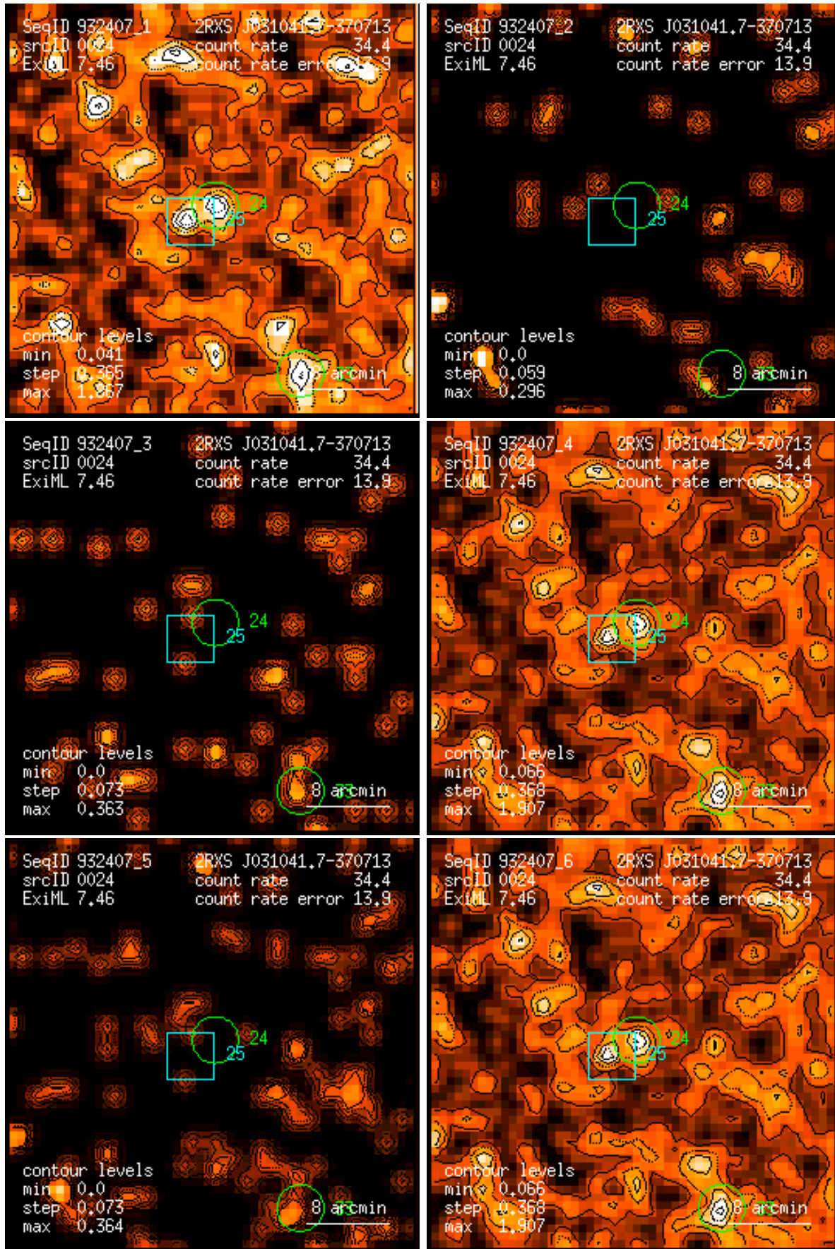
Figure 24: RASS 932407: detection 0024: band rate images, Gaussian filter: (1) PSPC channels 11 – 41, (2) 52 – 90, (3) 91 – 201, (4) 11 – 235, (5) 52 – 201, (6) 11 – 201. Broad band rates in counts/ks. Band rate contour levels in counts/ks/arcmin 2 .
