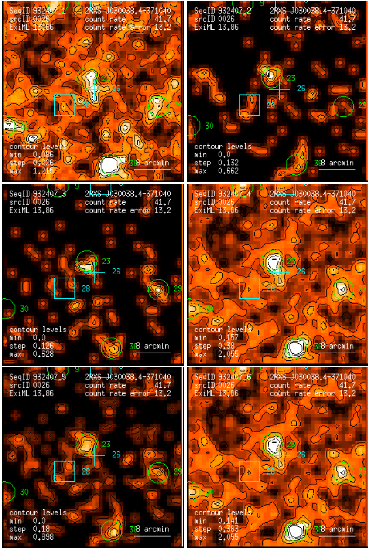
Figure 26: RASS 932407: detection 0026: band rate images, Gaussian filter: (1) PSPC channels 11 – 41, (2) 52 – 90, (3) 91 – 201, (4) 11 – 235, (5) 52 – 201, (6) 11 – 201. Broad band rates in counts/ks. Band rate contour levels in counts/ks/arcmin 2 .
