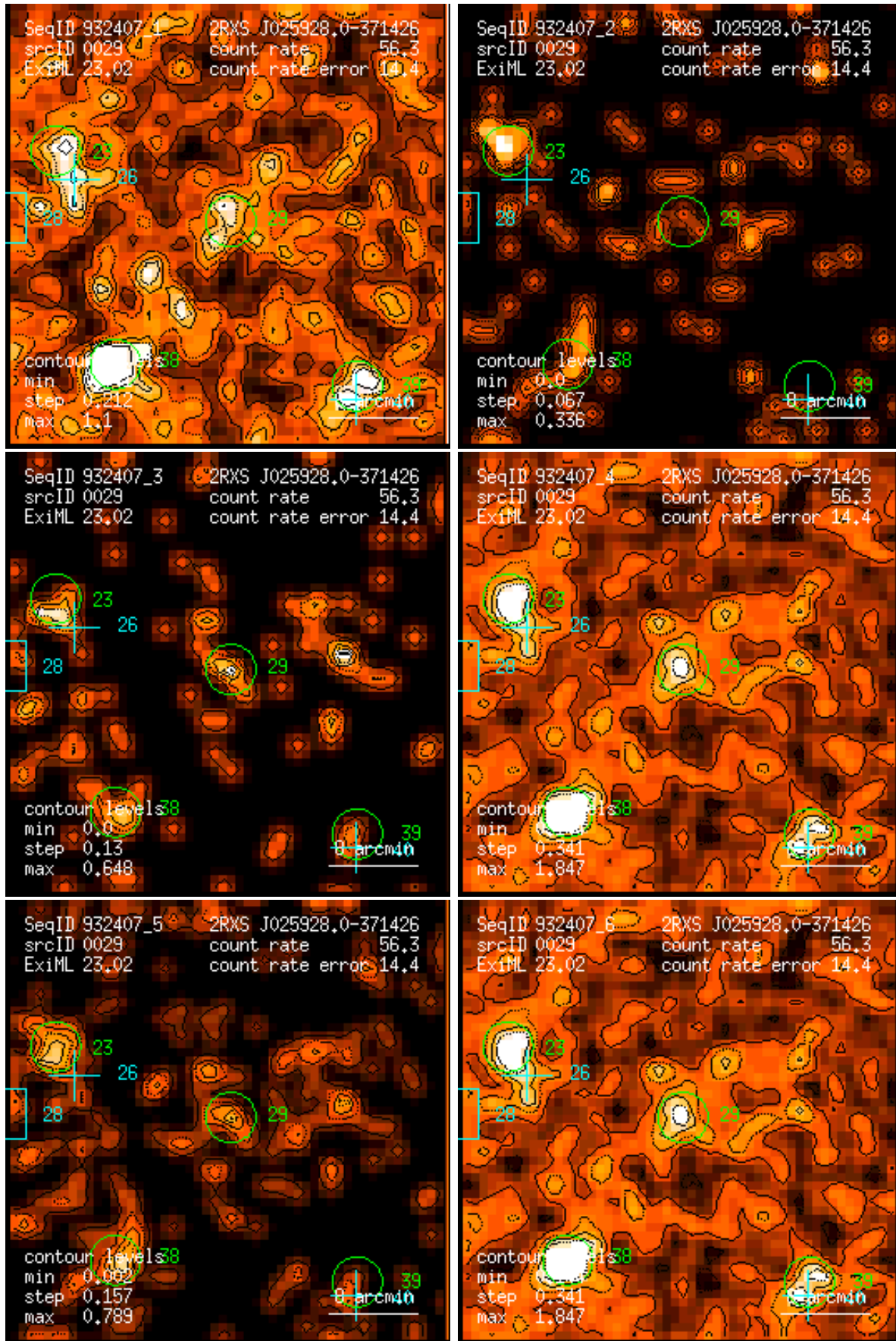
Figure 29: RASS 932407: detection 0029: band rate images, Gaussian filter: (1) PSPC channels 11 – 41, (2) 52 – 90, (3) 91 – 201, (4) 11 – 235, (5) 52 – 201, (6) 11 – 201. Broad band rates in counts/ks. Band rate contour levels in counts/ks/arcmin 2 .
