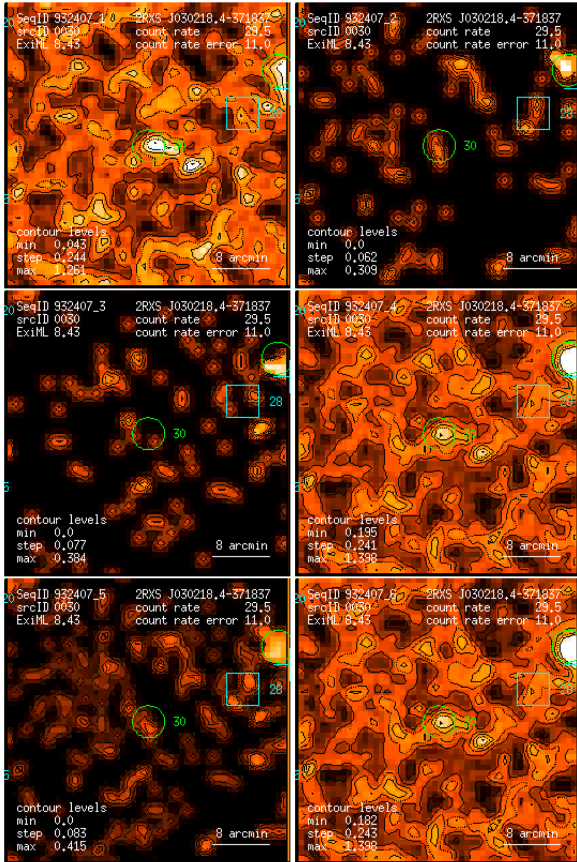
Figure 30: RASS 932407: detection 0030: band rate images, Gaussian filter: (1) PSPC channels 11 – 41, (2) 52 – 90, (3) 91 – 201, (4) 11 – 235, (5) 52 – 201, (6) 11 – 201. Broad band rates in counts/ks. Band rate contour levels in counts/ks/arcmin 2 .
