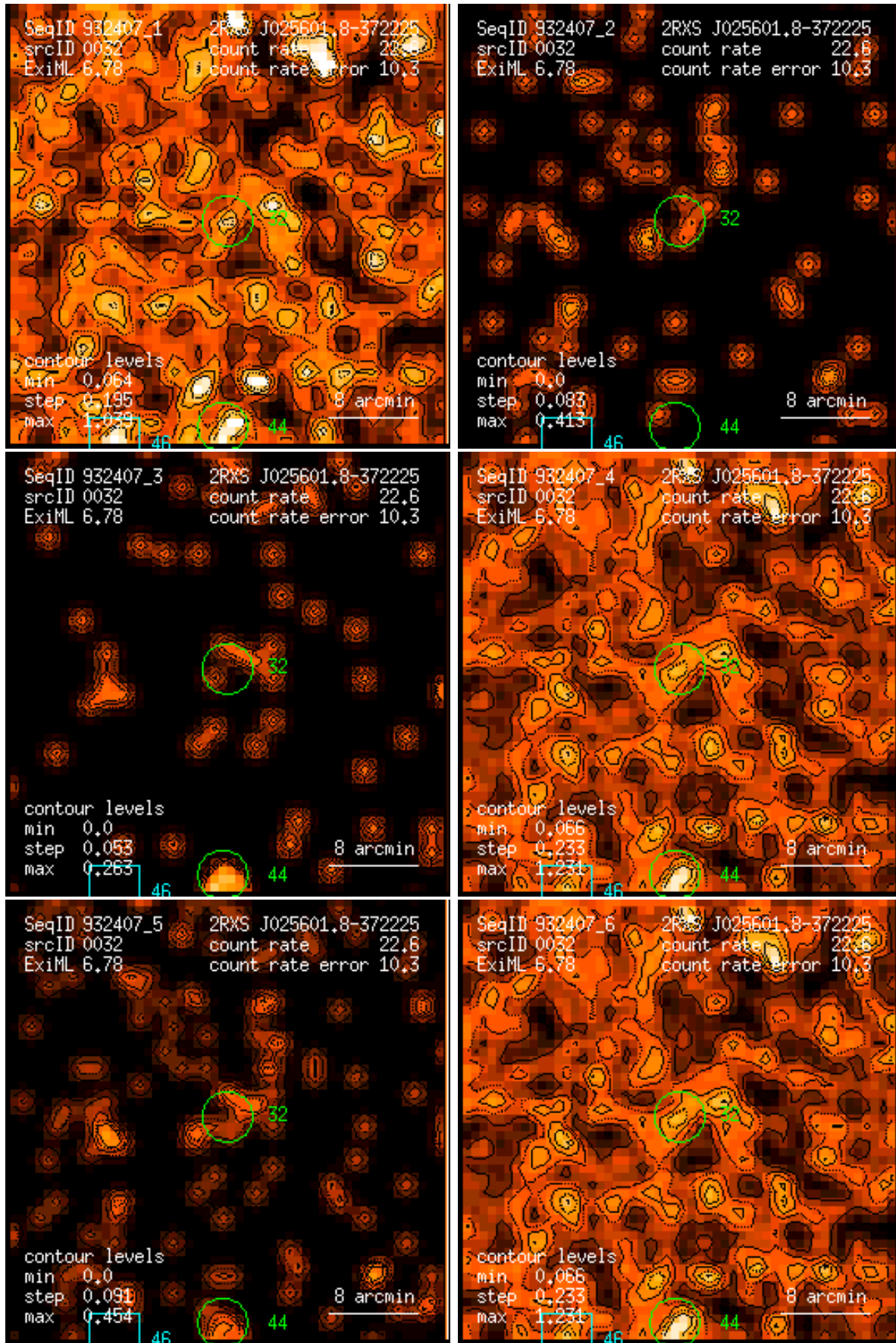
Figure 32: RASS 932407: detection 0032: band rate images, Gaussian filter: (1) PSPC channels 11 – 41, (2) 52 – 90, (3) 91 – 201, (4) 11 – 235, (5) 52 – 201, (6) 11 – 201. Broad band rates in counts/ks. Band rate contour levels in counts/ks/arcmin 2 .
