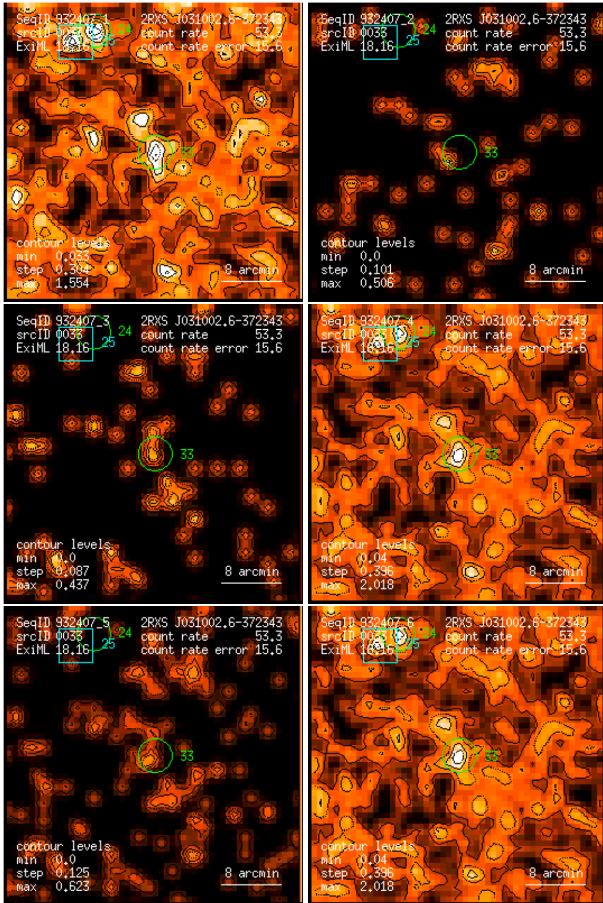
Figure 33: RASS 932407: detection 0033: band rate images, Gaussian filter: (1) PSPC channels 11 – 41, (2) 52 – 90, (3) 91 – 201, (4) 11 – 235, (5) 52 – 201, (6) 11 – 201. Broad band rates in counts/ks. Band rate contour levels in counts/ks/arcmin 2 .
