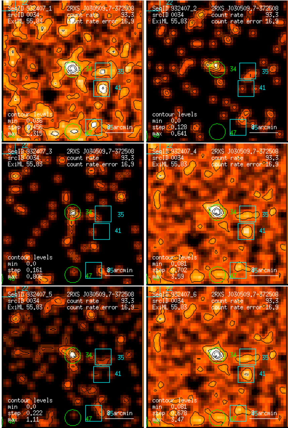
Figure 34: RASS 932407: detection 0034: band rate images, Gaussian filter: (1) PSPC channels 11 – 41, (2) 52 – 90, (3) 91 – 201, (4) 11 – 235, (5) 52 – 201, (6) 11 – 201. Broad band rates in counts/ks. Band rate contour levels in counts/ks/arcmin 2 .
