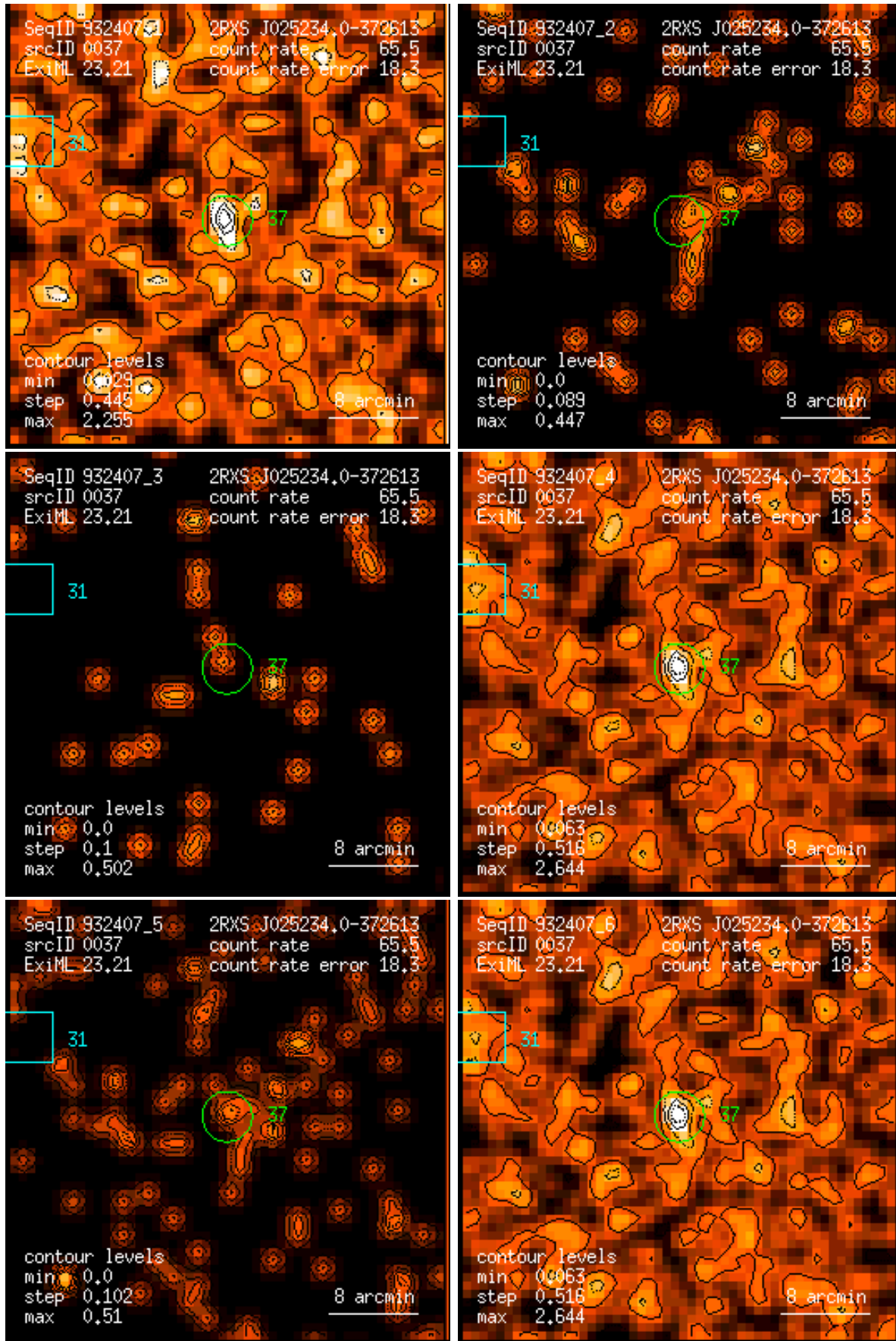
Figure 37: RASS 932407: detection 0037: band rate images, Gaussian filter: (1) PSPC channels 11 – 41, (2) 52 – 90, (3) 91 – 201, (4) 11 – 235, (5) 52 – 201, (6) 11 – 201. Broad band rates in counts/ks. Band rate contour levels in counts/ks/arcmin 2 .
