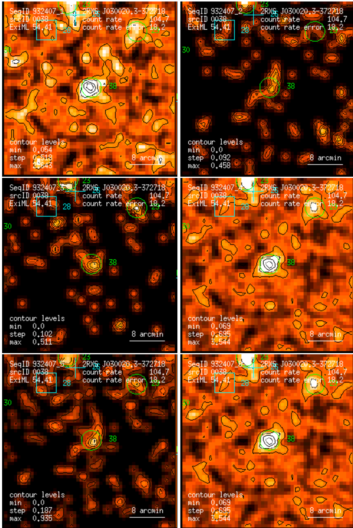
Figure 38: RASS 932407: detection 0038: band rate images, Gaussian filter: (1) PSPC channels 11 – 41, (2) 52 – 90, (3) 91 – 201, (4) 11 – 235, (5) 52 – 201, (6) 11 – 201. Broad band rates in counts/ks. Band rate contour levels in counts/ks/arcmin 2 .
