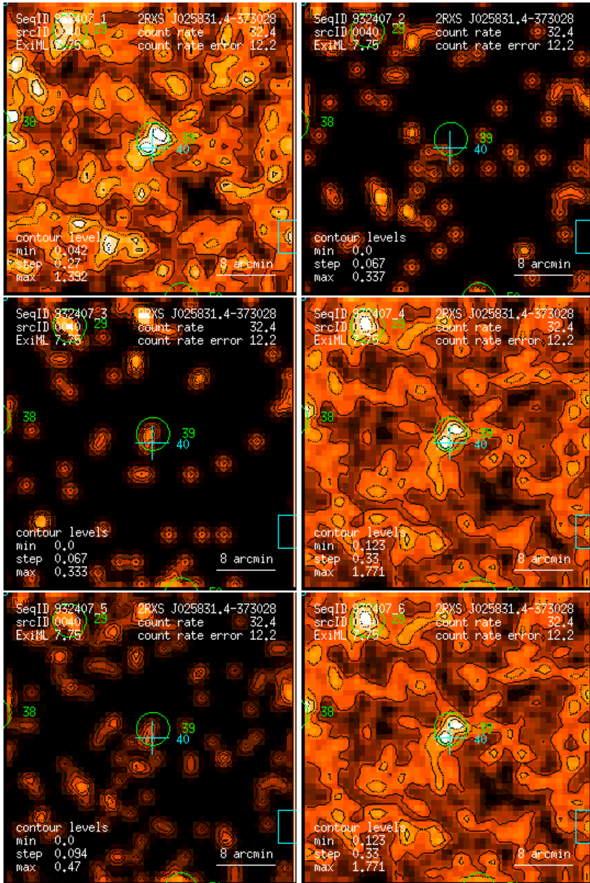
Figure 40: RASS 932407: detection 0040: band rate images, Gaussian filter: (1) PSPC channels 11 – 41, (2) 52 – 90, (3) 91 – 201, (4) 11 – 235, (5) 52 – 201, (6) 11 – 201. Broad band rates in counts/ks. Band rate contour levels in counts/ks/arcmin 2 .
