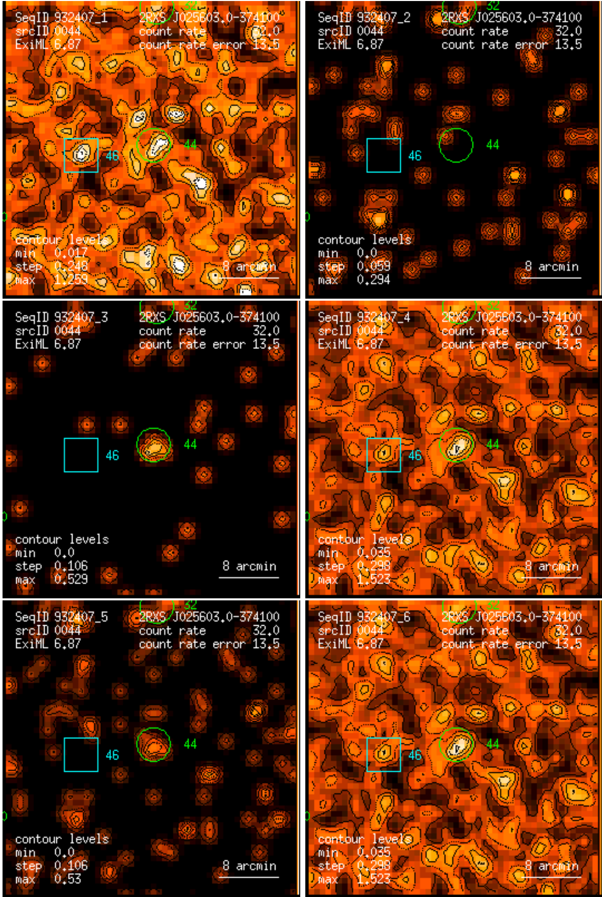
Figure 44: RASS 932407: detection 0044: band rate images, Gaussian filter: (1) PSPC channels 11 – 41, (2) 52 – 90, (3) 91 – 201, (4) 11 – 235, (5) 52 – 201, (6) 11 – 201. Broad band rates in counts/ks. Band rate contour levels in counts/ks/arcmin 2 .
