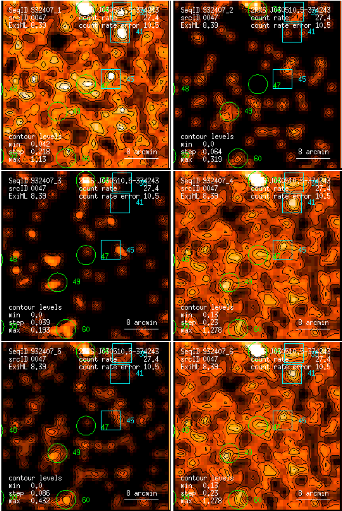
Figure 47: RASS 932407: detection 0047: band rate images, Gaussian filter: (1) PSPC channels 11 – 41, (2) 52 – 90, (3) 91 – 201, (4) 11 – 235, (5) 52 – 201, (6) 11 – 201. Broad band rates in counts/ks. Band rate contour levels in counts/ks/arcmin 2 .
