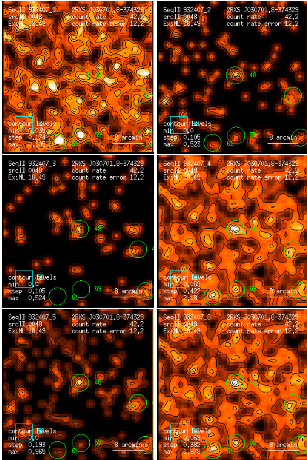
Figure 48: RASS 932407: detection 0048: band rate images, Gaussian filter: (1) PSPC channels 11 – 41, (2) 52 – 90, (3) 91 – 201, (4) 11 – 235, (5) 52 – 201, (6) 11 – 201. Broad band rates in counts/ks. Band rate contour levels in counts/ks/arcmin 2 .
