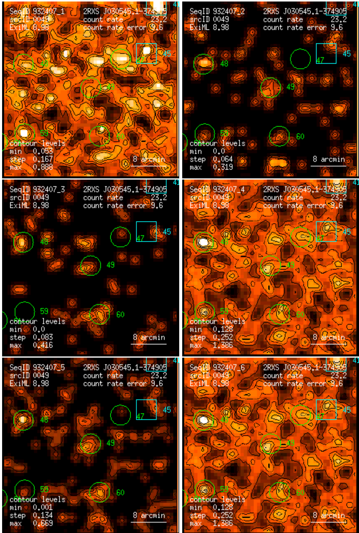
Figure 49: RASS 932407: detection 0049: band rate images, Gaussian filter: (1) PSPC channels 11 – 41, (2) 52 – 90, (3) 91 – 201, (4) 11 – 235, (5) 52 – 201, (6) 11 – 201. Broad band rates in counts/ks. Band rate contour levels in counts/ks/arcmin 2 .
