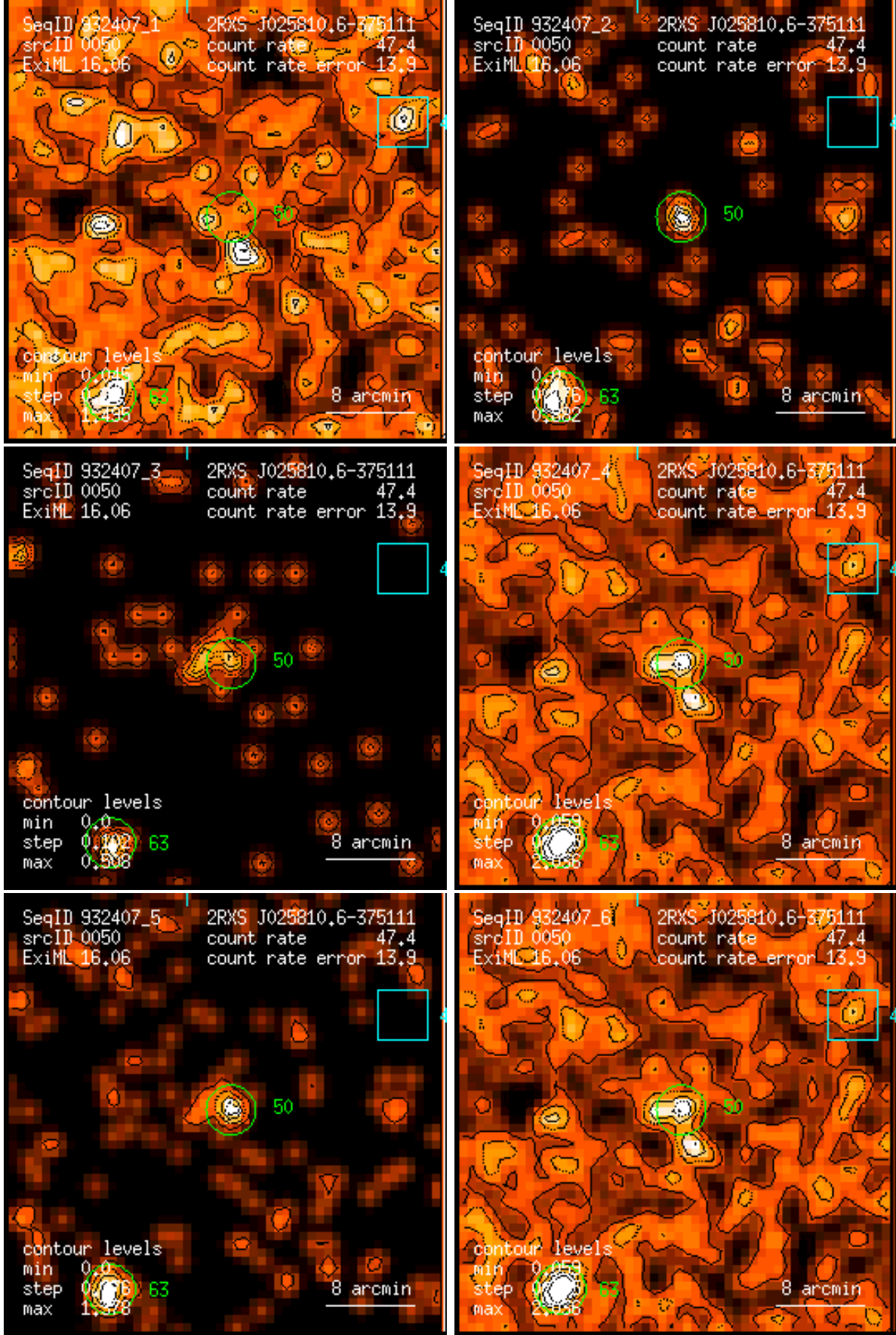
Figure 50: RASS 932407: detection 0050: band rate images, Gaussian filter: (1) PSPC channels 11 – 41, (2) 52 – 90, (3) 91 – 201, (4) 11 – 235, (5) 52 – 201, (6) 11 – 201. Broad band rates in counts/ks. Band rate contour levels in counts/ks/arcmin 2 .
