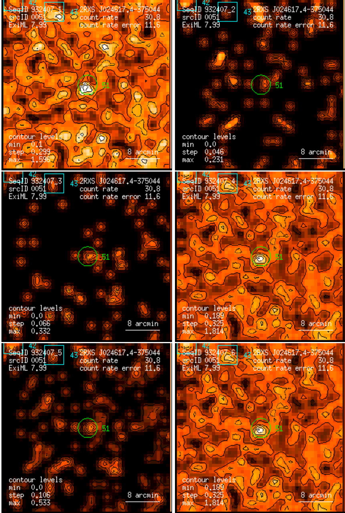
Figure 51: RASS 932407: detection 0051: band rate images, Gaussian filter: (1) PSPC channels 11 – 41, (2) 52 – 90, (3) 91 – 201, (4) 11 – 235, (5) 52 – 201, (6) 11 – 201. Broad band rates in counts/ks. Band rate contour levels in counts/ks/arcmin 2 .
