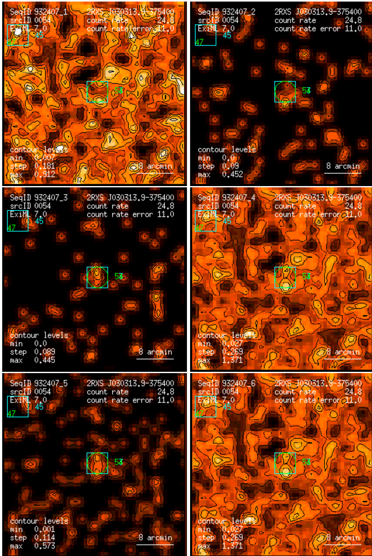
Figure 54: RASS 932407: detection 0054: band rate images, Gaussian filter: (1) PSPC channels 11 – 41, (2) 52 – 90, (3) 91 – 201, (4) 11 – 235, (5) 52 – 201, (6) 11 – 201. Broad band rates in counts/ks. Band rate contour levels in counts/ks/arcmin 2 .
