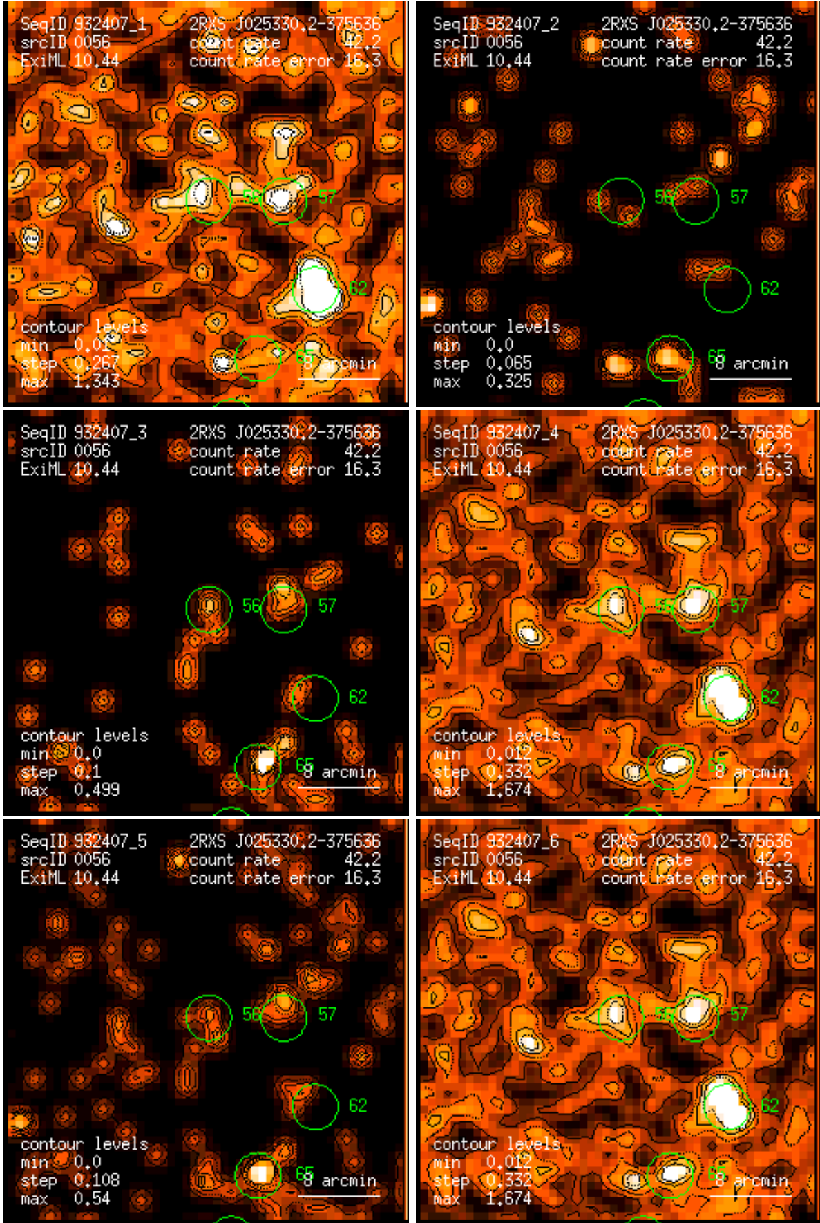
Figure 56: RASS 932407: detection 0056: band rate images, Gaussian filter: (1) PSPC channels 11 – 41, (2) 52 – 90, (3) 91 – 201, (4) 11 – 235, (5) 52 – 201, (6) 11 – 201. Broad band rates in counts/ks. Band rate contour levels in counts/ks/arcmin 2 .
