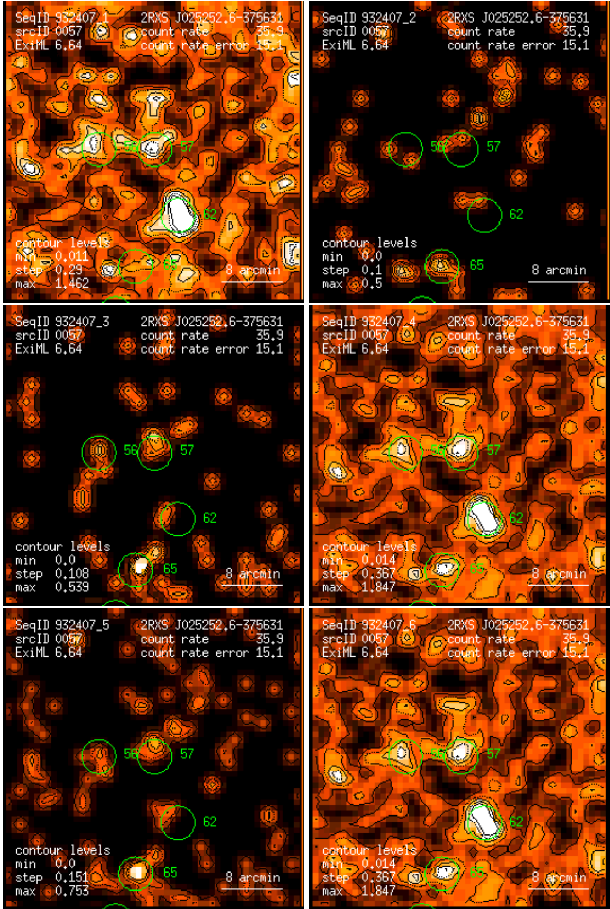
Figure 57: RASS 932407: detection 0057: band rate images, Gaussian filter: (1) PSPC channels 11 – 41, (2) 52 – 90, (3) 91 – 201, (4) 11 – 235, (5) 52 – 201, (6) 11 – 201. Broad band rates in counts/ks. Band rate contour levels in counts/ks/arcmin 2 .
