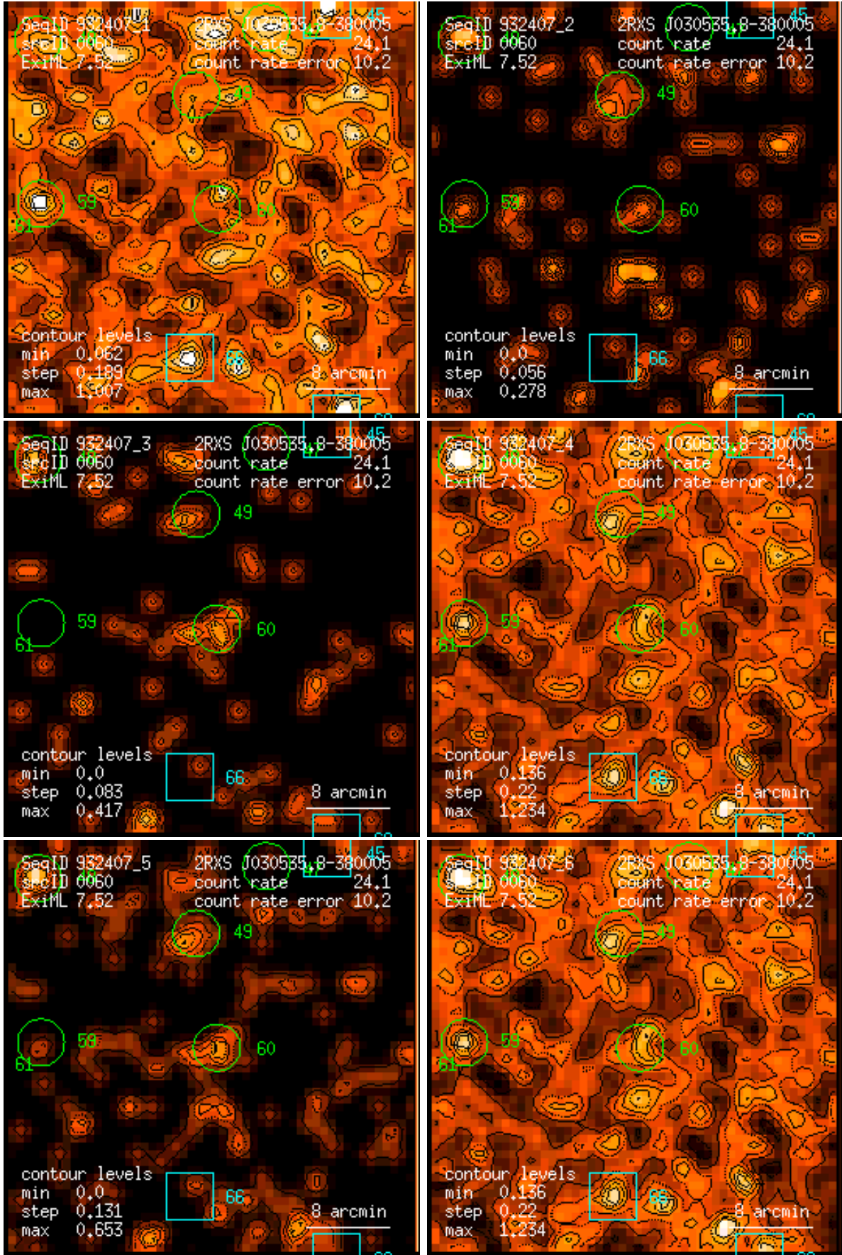
Figure 60: RASS 932407: detection 0060: band rate images, Gaussian filter: (1) PSPC channels 11 – 41, (2) 52 – 90, (3) 91 – 201, (4) 11 – 235, (5) 52 – 201, (6) 11 – 201. Broad band rates in counts/ks. Band rate contour levels in counts/ks/arcmin 2 .
