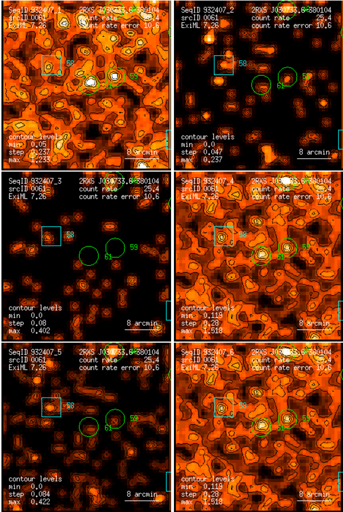
Figure 61: RASS 932407: detection 0061: band rate images, Gaussian filter: (1) PSPC channels 11 – 41, (2) 52 – 90, (3) 91 – 201, (4) 11 – 235, (5) 52 – 201, (6) 11 – 201. Broad band rates in counts/ks. Band rate contour levels in counts/ks/arcmin 2 .
