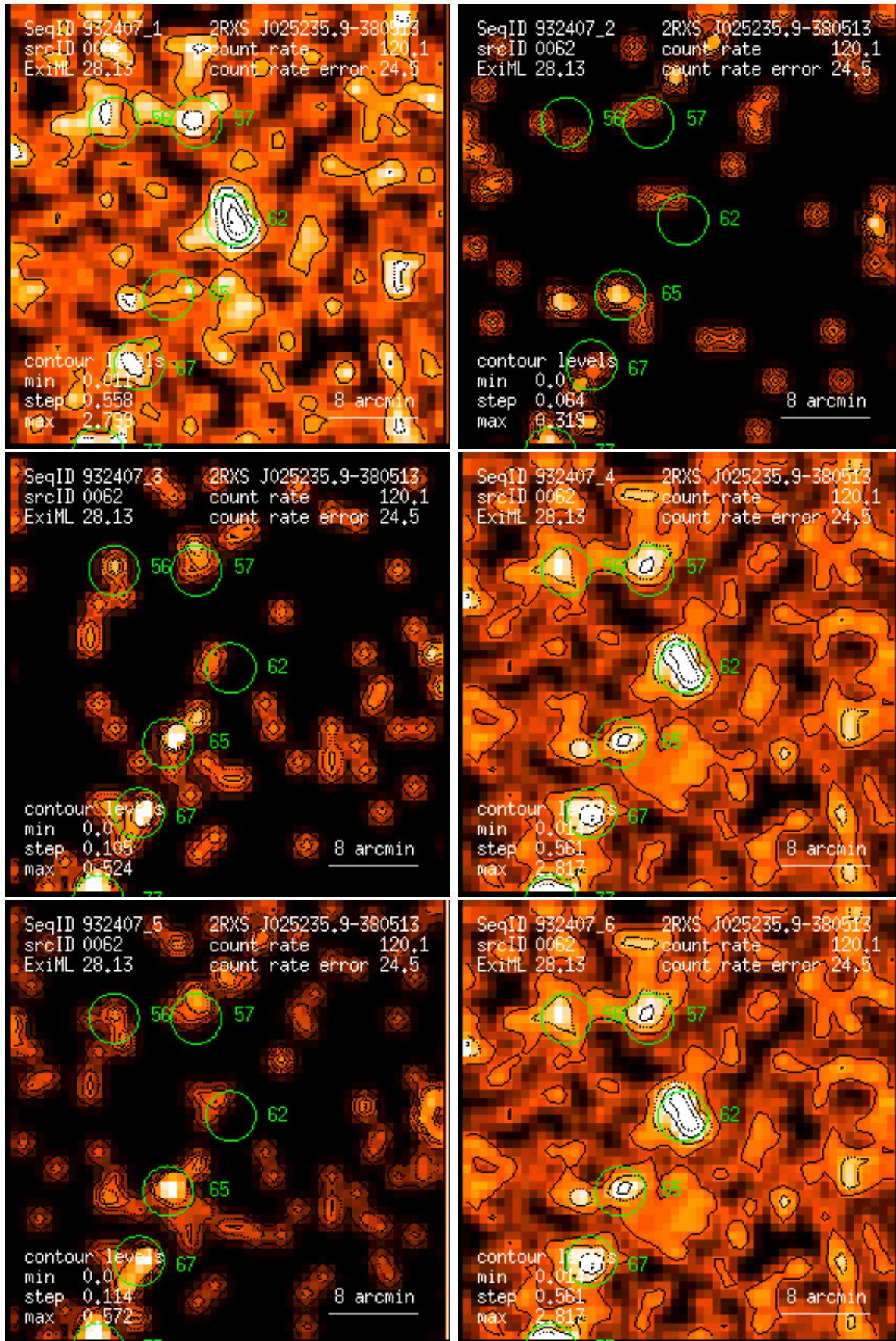
Figure 62: RASS 932407: detection 0062: band rate images, Gaussian filter: (1) PSPC channels 11 – 41, (2) 52 – 90, (3) 91 – 201, (4) 11 – 235, (5) 52 – 201, (6) 11 – 201. Broad band rates in counts/ks. Band rate contour levels in counts/ks/arcmin 2 .
