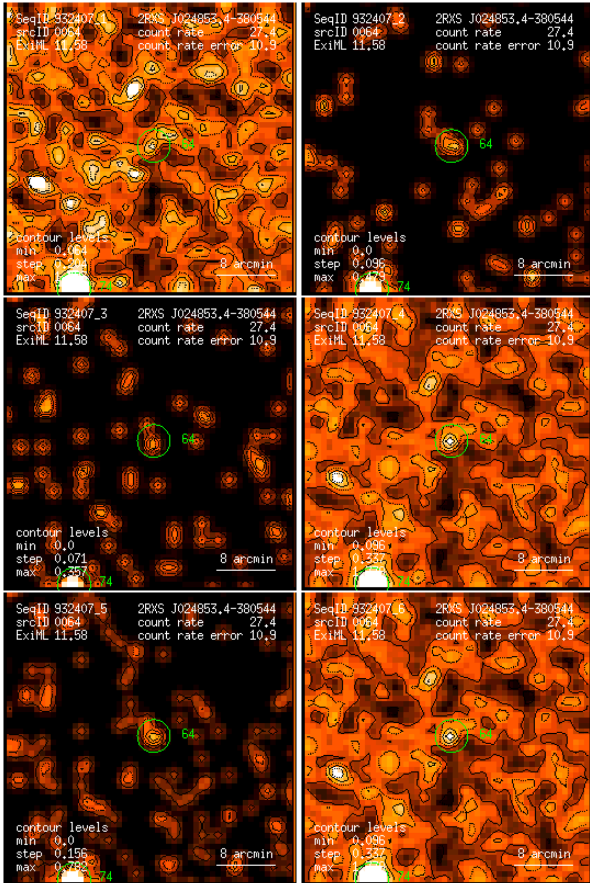
Figure 64: RASS 932407: detection 0064: band rate images, Gaussian filter: (1) PSPC channels 11 – 41, (2) 52 – 90, (3) 91 – 201, (4) 11 – 235, (5) 52 – 201, (6) 11 – 201. Broad band rates in counts/ks. Band rate contour levels in counts/ks/arcmin 2 .
