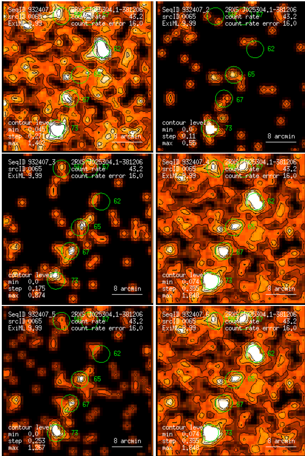
Figure 65: RASS 932407: detection 0065: band rate images, Gaussian filter: (1) PSPC channels 11 – 41, (2) 52 – 90, (3) 91 – 201, (4) 11 – 235, (5) 52 – 201, (6) 11 – 201. Broad band rates in counts/ks. Band rate contour levels in counts/ks/arcmin 2 .
