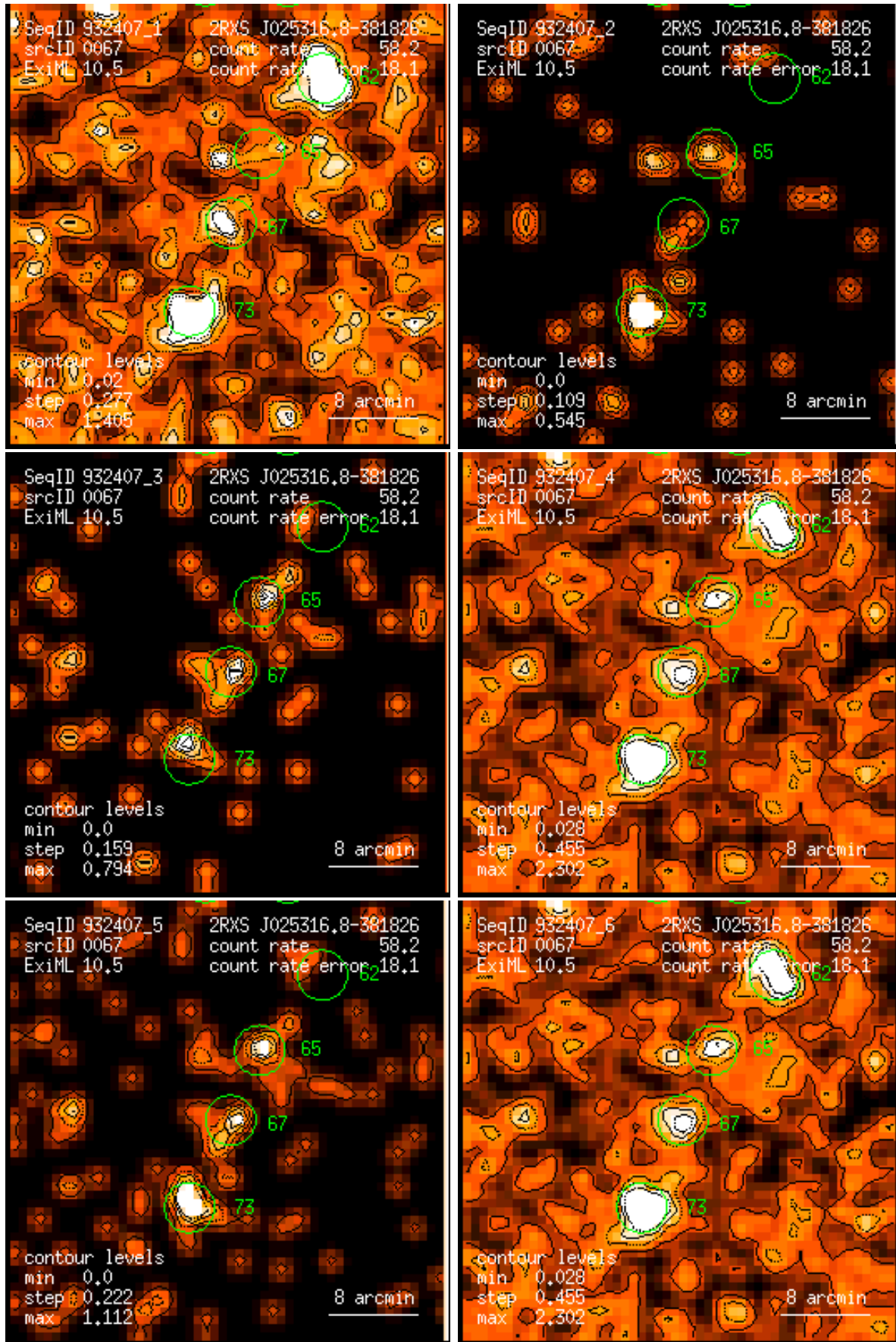
Figure 67: RASS 932407: detection 0067: band rate images, Gaussian filter: (1) PSPC channels 11 – 41, (2) 52 – 90, (3) 91 – 201, (4) 11 – 235, (5) 52 – 201, (6) 11 – 201. Broad band rates in counts/ks. Band rate contour levels in counts/ks/arcmin 2 .
