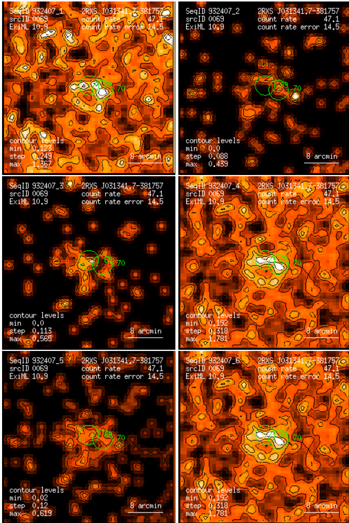
Figure 69: RASS 932407: detection 0069: band rate images, Gaussian filter: (1) PSPC channels 11 – 41, (2) 52 – 90, (3) 91 – 201, (4) 11 – 235, (5) 52 – 201, (6) 11 – 201. Broad band rates in counts/ks. Band rate contour levels in counts/ks/arcmin 2 .
