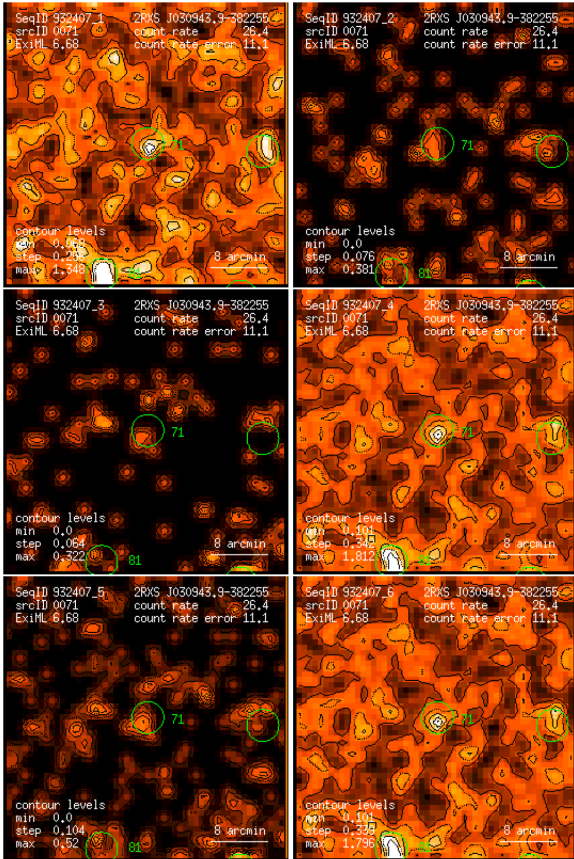
Figure 71: RASS 932407: detection 0071: band rate images, Gaussian filter: (1) PSPC channels 11 – 41, (2) 52 – 90, (3) 91 – 201, (4) 11 – 235, (5) 52 – 201, (6) 11 – 201. Broad band rates in counts/ks. Band rate contour levels in counts/ks/arcmin 2 .
