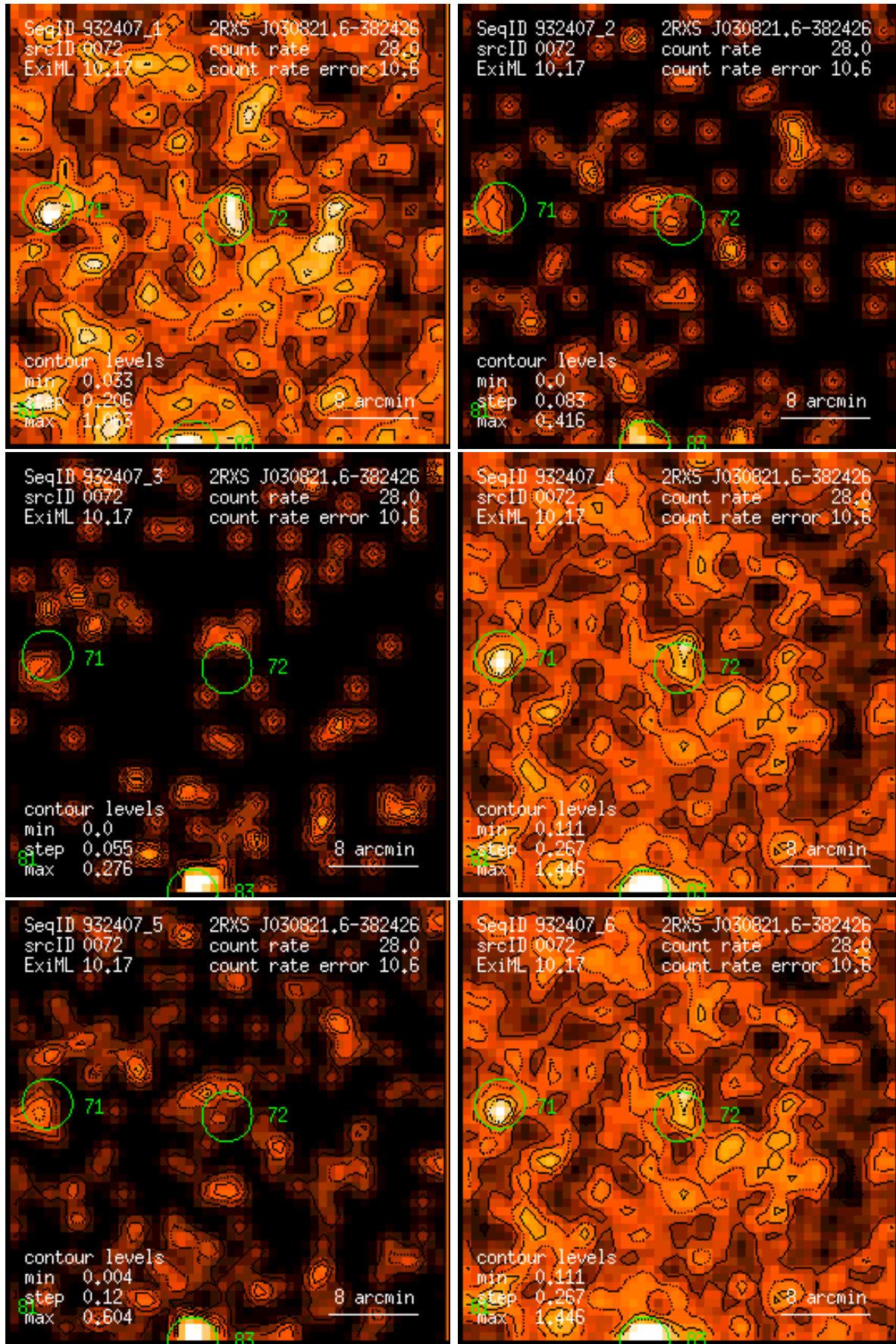
Figure 72: RASS 932407: detection 0072: band rate images, Gaussian filter: (1) PSPC channels 11 – 41, (2) 52 – 90, (3) 91 – 201, (4) 11 – 235, (5) 52 – 201, (6) 11 – 201. Broad band rates in counts/ks. Band rate contour levels in counts/ks/arcmin 2 .
