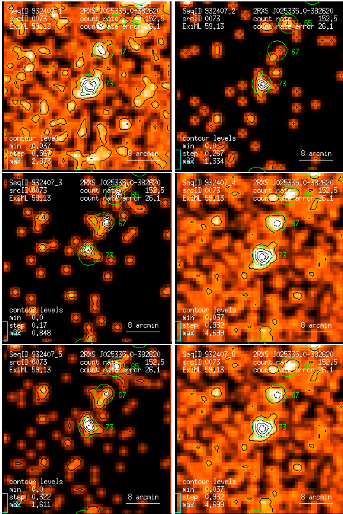
Figure 73: RASS 932407: detection 0073: band rate images, Gaussian filter: (1) PSPC channels 11 – 41, (2) 52 – 90, (3) 91 – 201, (4) 11 – 235, (5) 52 – 201, (6) 11 – 201. Broad band rates in counts/ks. Band rate contour levels in counts/ks/arcmin 2 .
