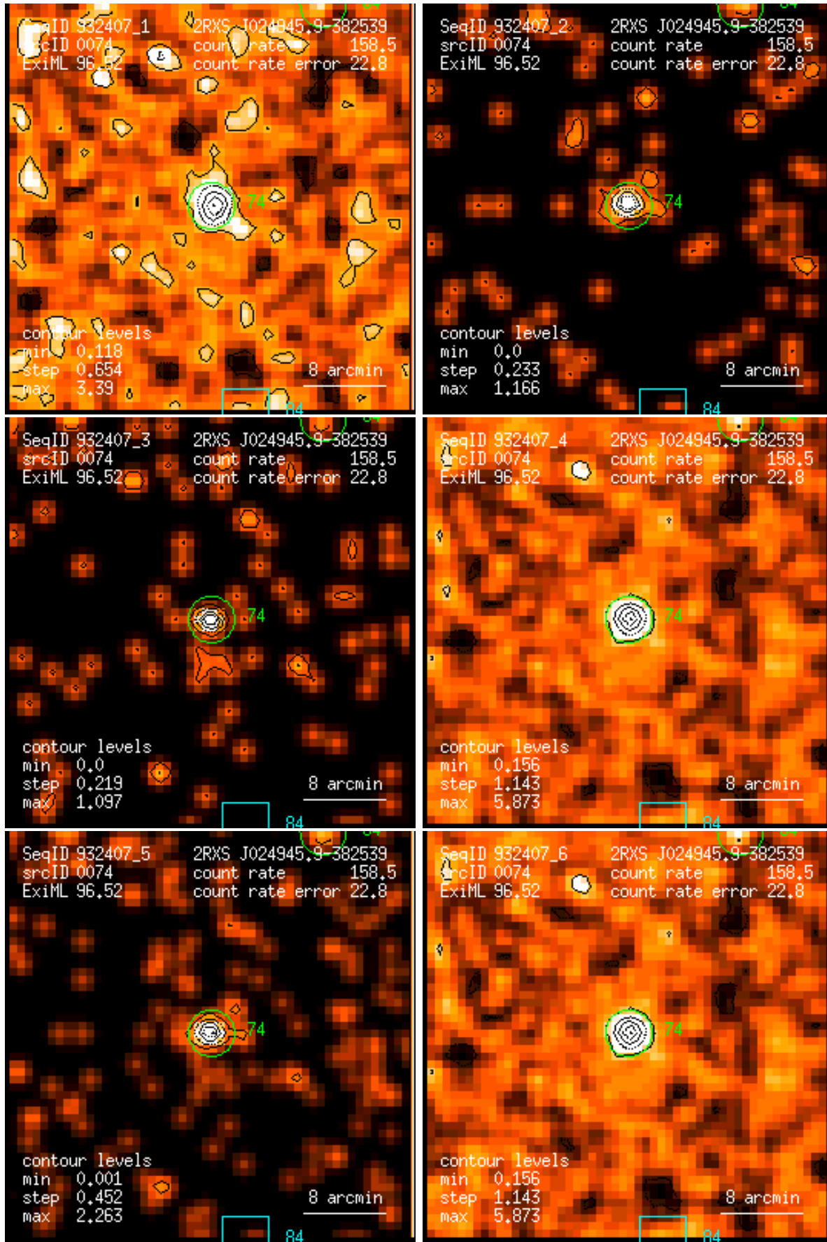
Figure 74: RASS 932407: detection 0074: band rate images, Gaussian filter: (1) PSPC channels 11 – 41, (2) 52 – 90, (3) 91 – 201, (4) 11 – 235, (5) 52 – 201, (6) 11 – 201. Broad band rates in counts/ks. Band rate contour levels in counts/ks/arcmin 2 .
