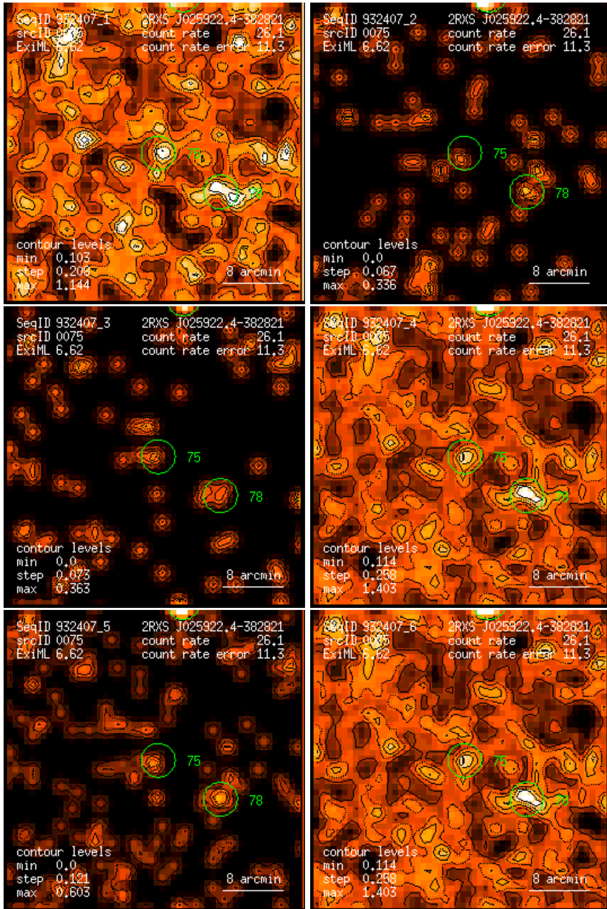
Figure 75: RASS 932407: detection 0075: band rate images, Gaussian filter: (1) PSPC channels 11 – 41, (2) 52 – 90, (3) 91 – 201, (4) 11 – 235, (5) 52 – 201, (6) 11 – 201. Broad band rates in counts/ks. Band rate contour levels in counts/ks/arcmin 2 .
