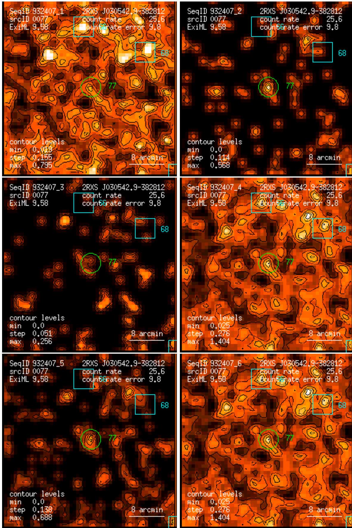
Figure 77: RASS 932407: detection 0077: band rate images, Gaussian filter: (1) PSPC channels 11 – 41, (2) 52 – 90, (3) 91 – 201, (4) 11 – 235, (5) 52 – 201, (6) 11 – 201. Broad band rates in counts/ks. Band rate contour levels in counts/ks/arcmin 2 .
