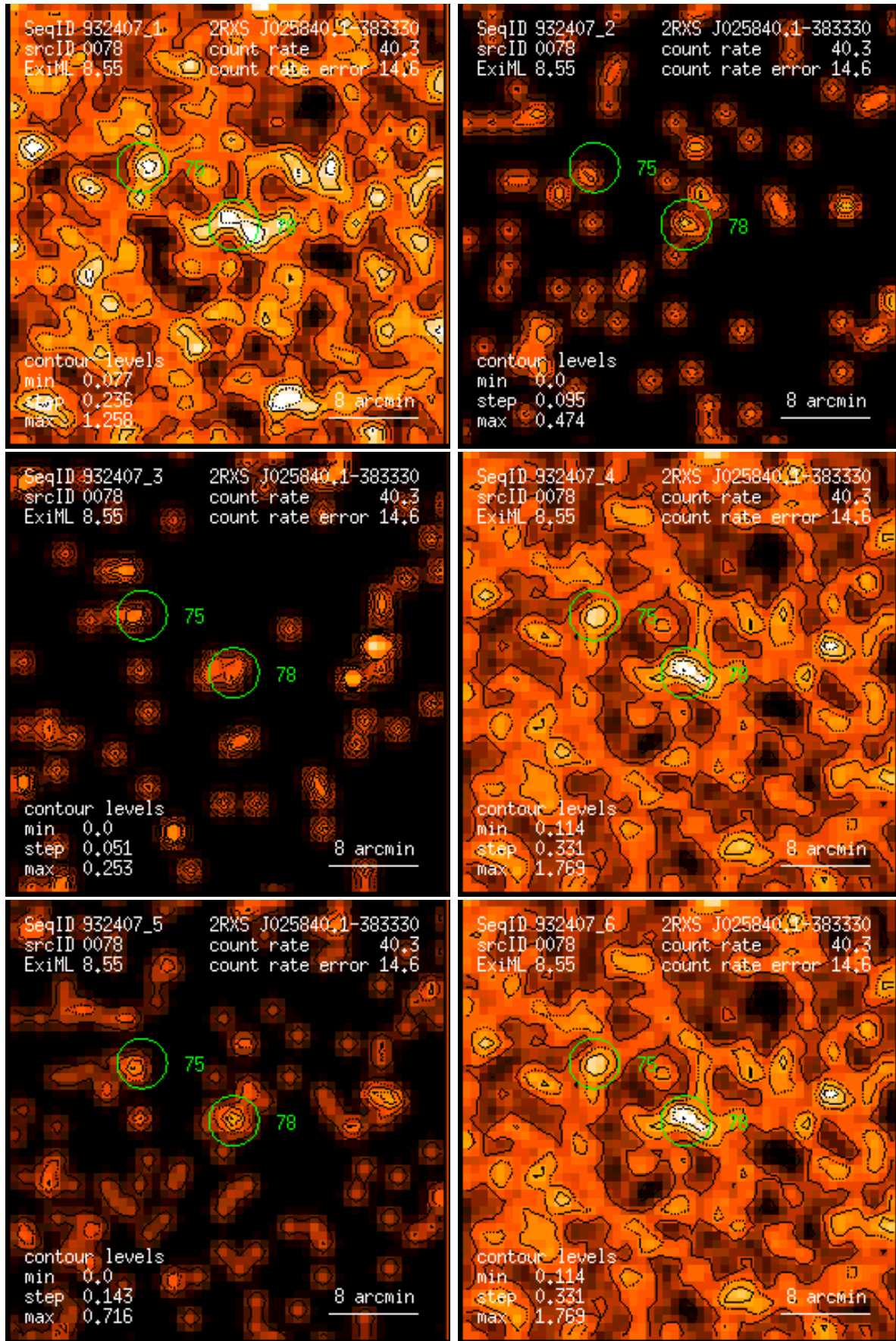
Figure 78: RASS 932407: detection 0078: band rate images, Gaussian filter: (1) PSPC channels 11 – 41, (2) 52 – 90, (3) 91 – 201, (4) 11 – 235, (5) 52 – 201, (6) 11 – 201. Broad band rates in counts/ks. Band rate contour levels in counts/ks/arcmin 2 .
