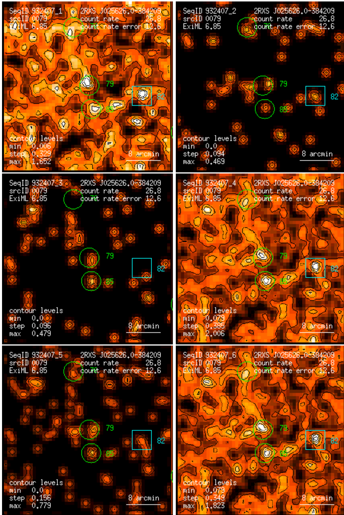
Figure 79: RASS 932407: detection 0079: band rate images, Gaussian filter: (1) PSPC channels 11 – 41, (2) 52 – 90, (3) 91 – 201, (4) 11 – 235, (5) 52 – 201, (6) 11 – 201. Broad band rates in counts/ks. Band rate contour levels in counts/ks/arcmin 2 .
