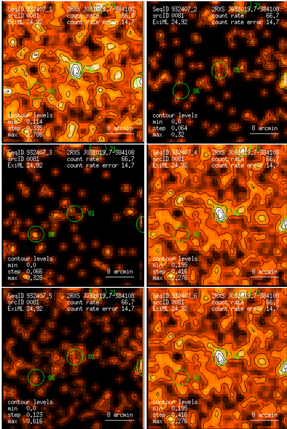
Figure 81: RASS 932407: detection 0081: band rate images, Gaussian filter: (1) PSPC channels 11 – 41, (2) 52 – 90, (3) 91 – 201, (4) 11 – 235, (5) 52 – 201, (6) 11 – 201. Broad band rates in counts/ks. Band rate contour levels in counts/ks/arcmin 2 .
