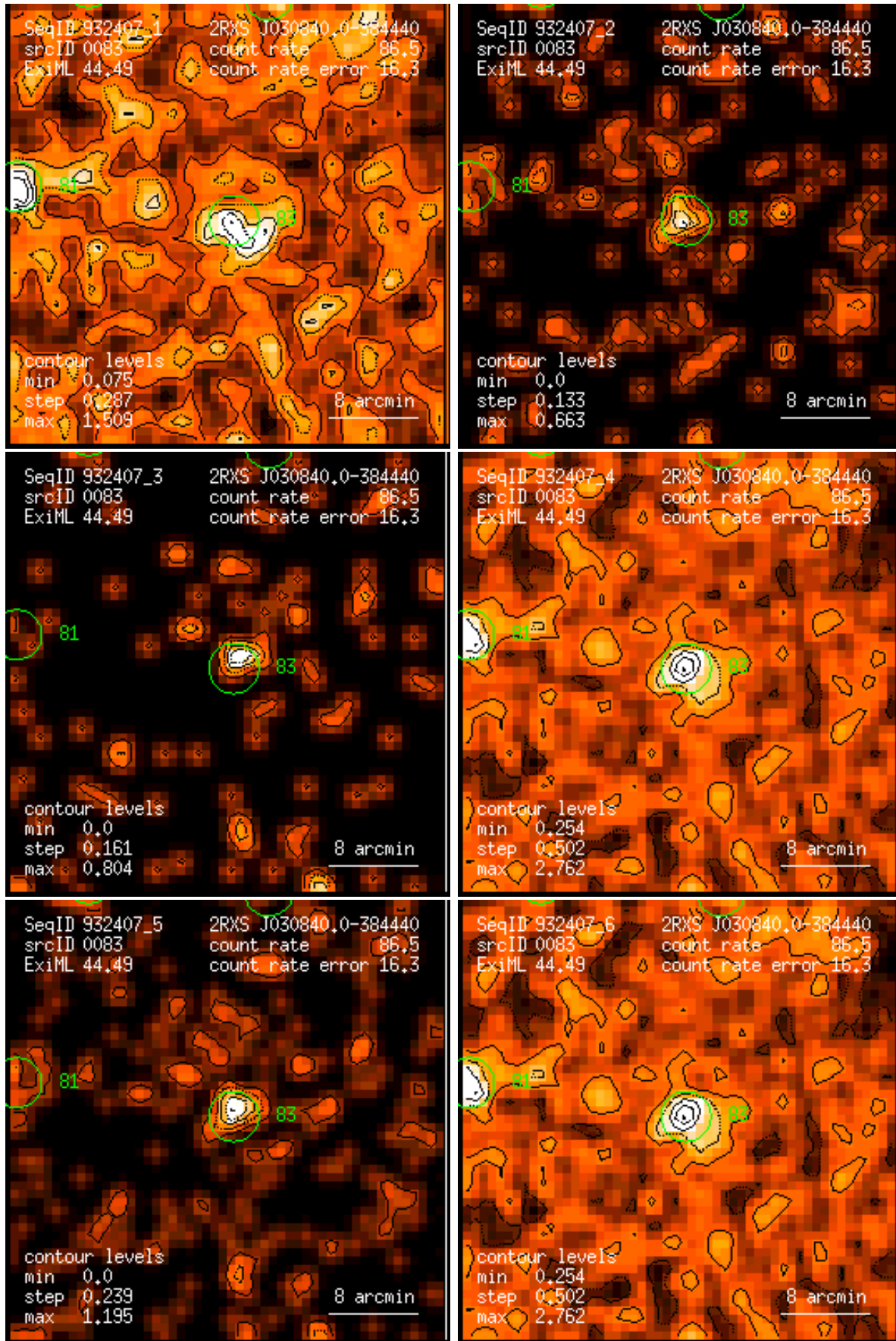
Figure 83: RASS 932407: detection 0083: band rate images, Gaussian filter: (1) PSPC channels 11 – 41, (2) 52 – 90, (3) 91 – 201, (4) 11 – 235, (5) 52 – 201, (6) 11 – 201. Broad band rates in counts/ks. Band rate contour levels in counts/ks/arcmin 2 .
