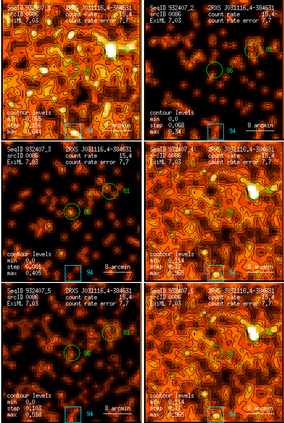
Figure 86: RASS 932407: detection 0086: band rate images, Gaussian filter: (1) PSPC channels 11 – 41, (2) 52 – 90, (3) 91 – 201, (4) 11 – 235, (5) 52 – 201, (6) 11 – 201. Broad band rates in counts/ks. Band rate contour levels in counts/ks/arcmin 2 .
