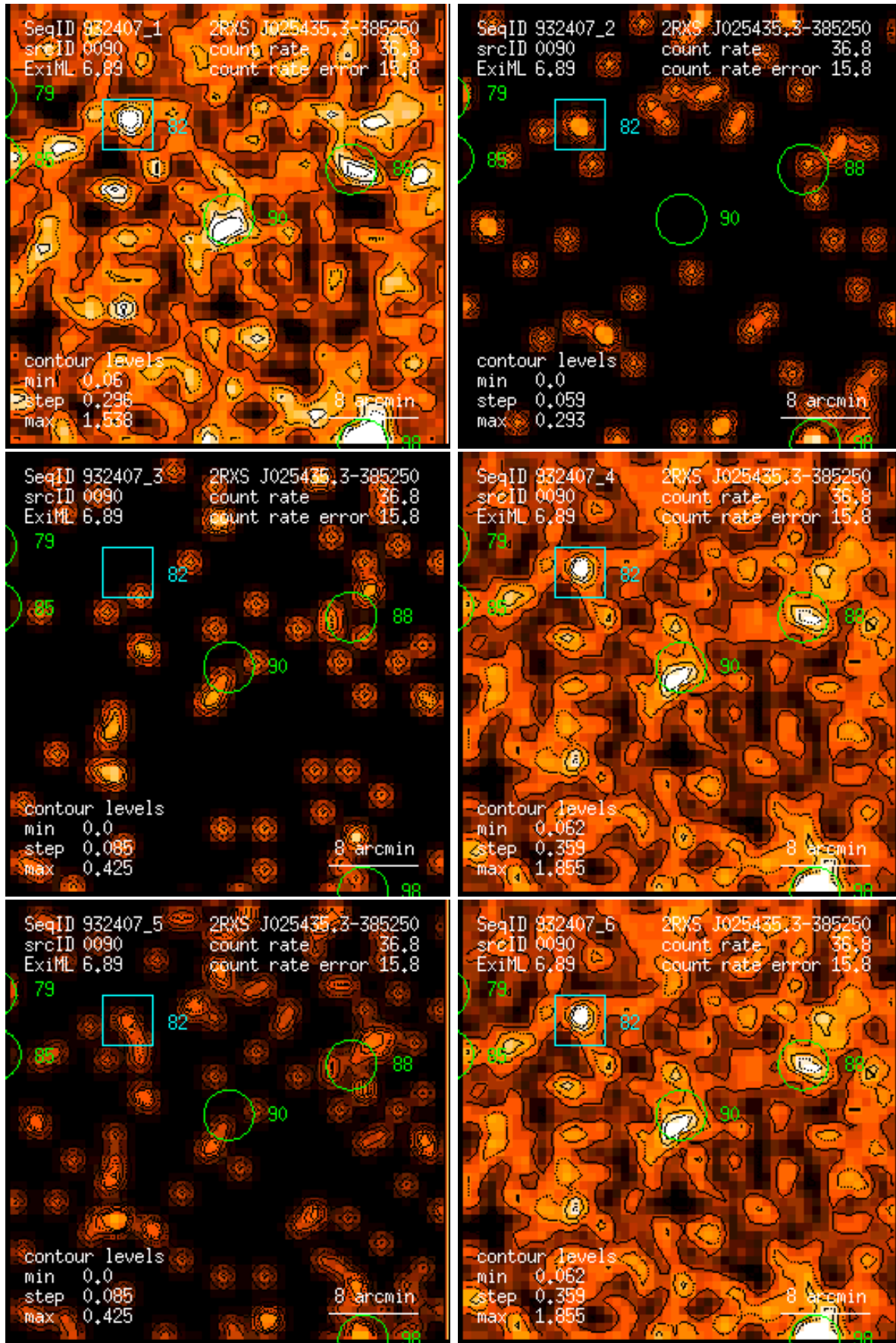
Figure 90: RASS 932407: detection 0090: band rate images, Gaussian filter: (1) PSPC channels 11 – 41, (2) 52 – 90, (3) 91 – 201, (4) 11 – 235, (5) 52 – 201, (6) 11 – 201. Broad band rates in counts/ks. Band rate contour levels in counts/ks/arcmin 2 .
