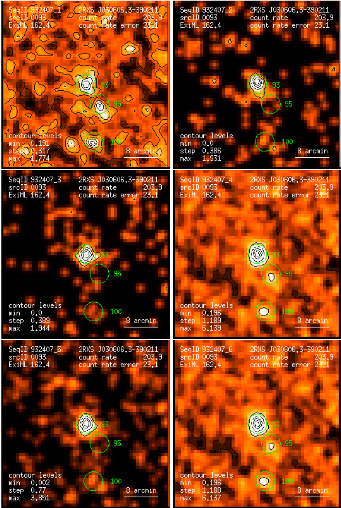
Figure 93: RASS 932407: detection 0093: band rate images, Gaussian filter: (1) PSPC channels 11 – 41, (2) 52 – 90, (3) 91 – 201, (4) 11 – 235, (5) 52 – 201, (6) 11 – 201. Broad band rates in counts/ks. Band rate contour levels in counts/ks/arcmin 2 .
