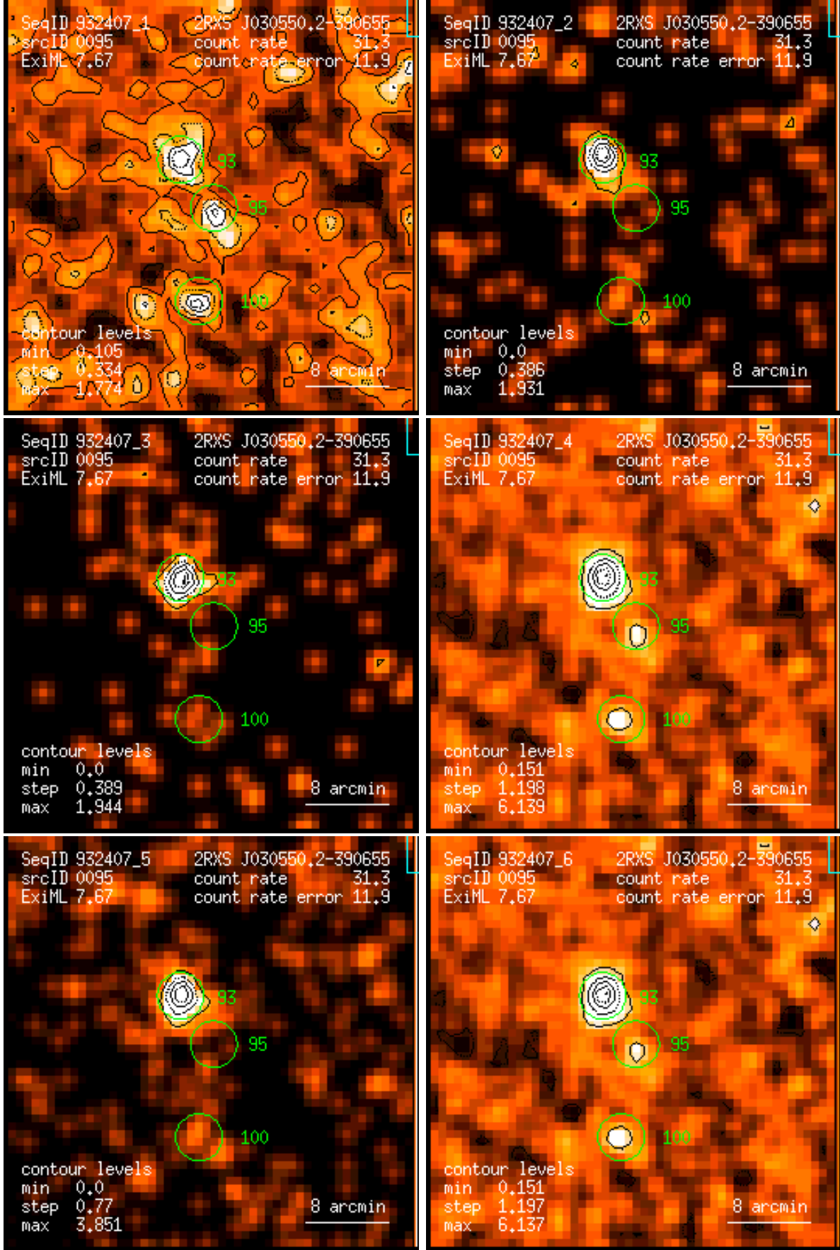
Figure 95: RASS 932407: detection 0095: band rate images, Gaussian filter: (1) PSPC channels 11 – 41, (2) 52 – 90, (3) 91 – 201, (4) 11 – 235, (5) 52 – 201, (6) 11 – 201. Broad band rates in counts/ks. Band rate contour levels in counts/ks/arcmin 2 .
