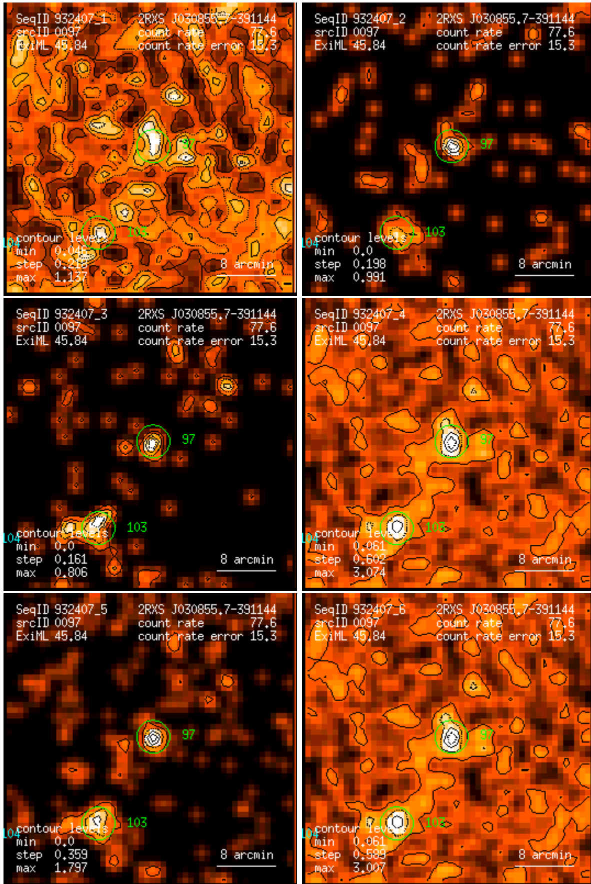
Figure 97: RASS 932407: detection 0097: band rate images, Gaussian filter: (1) PSPC channels 11 – 41, (2) 52 – 90, (3) 91 – 201, (4) 11 – 235, (5) 52 – 201, (6) 11 – 201. Broad band rates in counts/ks. Band rate contour levels in counts/ks/arcmin 2 .
