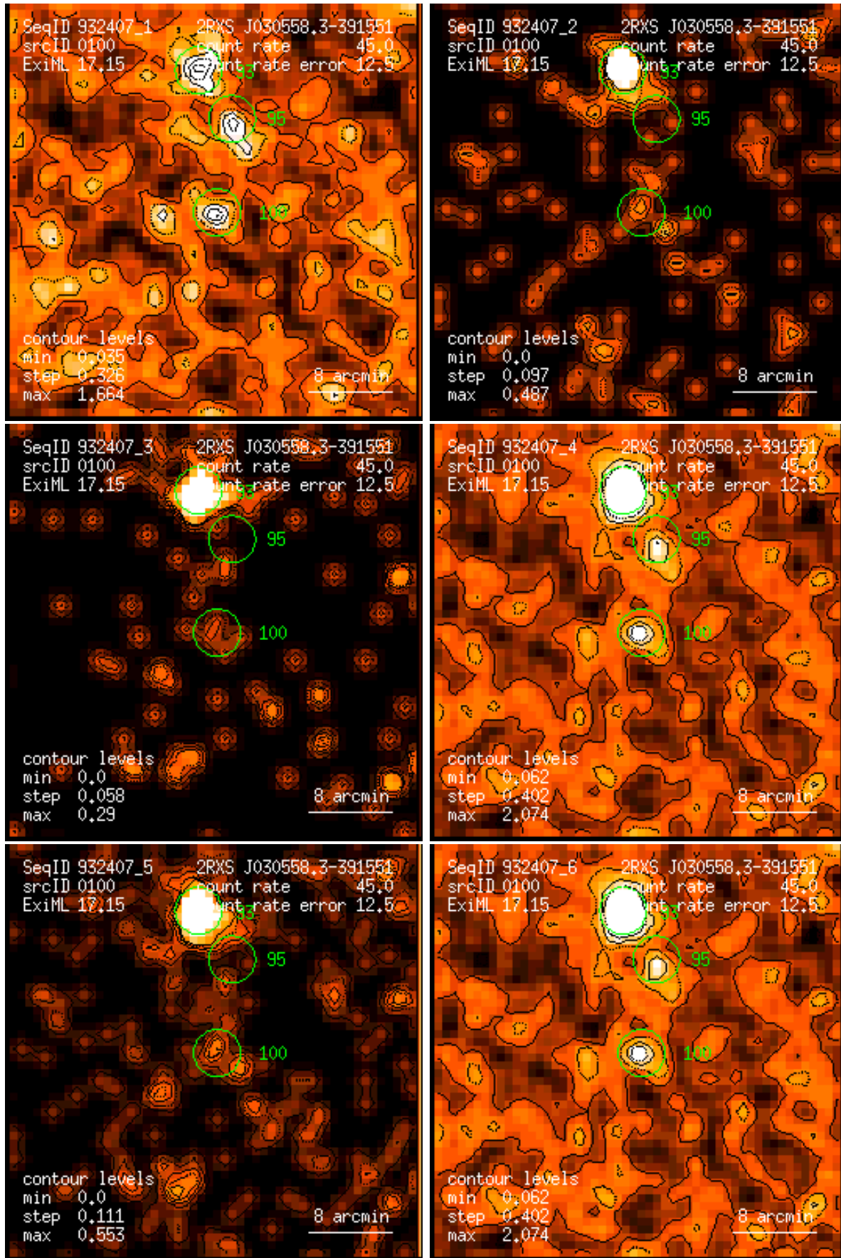
Figure 100: RASS 932407: detection 0100: band rate images, Gaussian filter: (1) PSPC channels 11 – 41, (2) 52 – 90, (3) 91 – 201, (4) 11 – 235, (5) 52 – 201, (6) 11 – 201. Broad band rates in counts/ks. Band rate contour levels in counts/ks/arcmin 2 .
