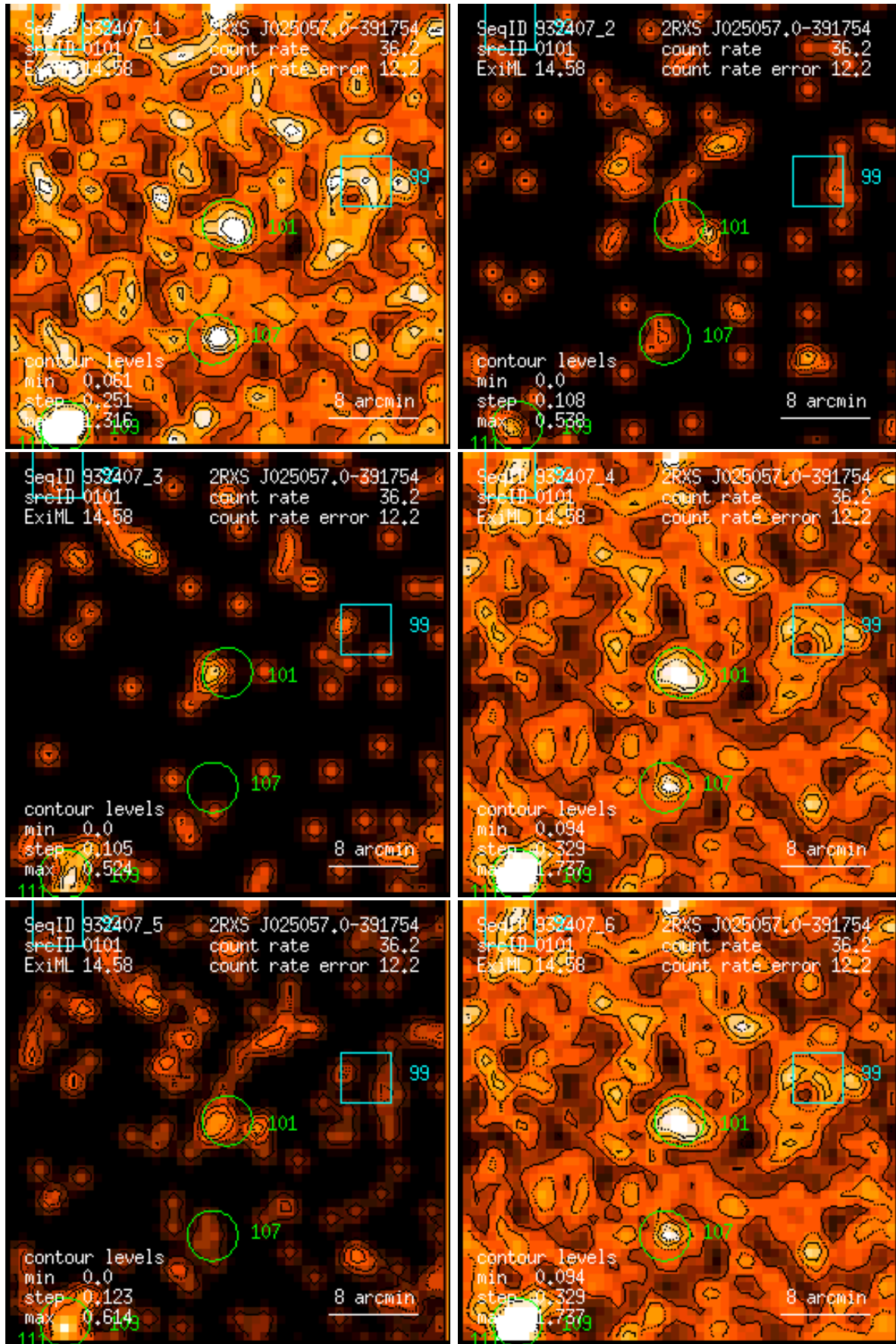
Figure 101: RASS 932407: detection 0101: band rate images, Gaussian filter: (1) PSPC channels 11 – 41, (2) 52 – 90, (3) 91 – 201, (4) 11 – 235, (5) 52 – 201, (6) 11 – 201. Broad band rates in counts/ks. Band rate contour levels in counts/ks/arcmin 2 .
