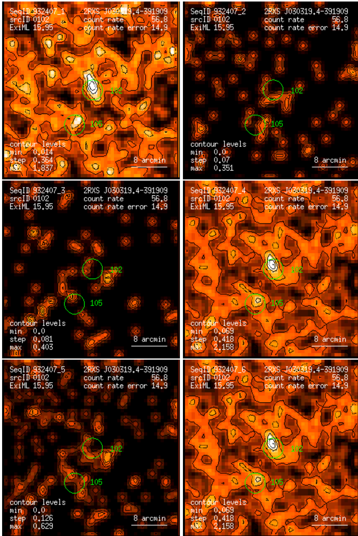
Figure 102: RASS 932407: detection 0102: band rate images, Gaussian filter: (1) PSPC channels 11 – 41, (2) 52 – 90, (3) 91 – 201, (4) 11 – 235, (5) 52 – 201, (6) 11 – 201. Broad band rates in counts/ks. Band rate contour levels in counts/ks/arcmin 2 .
