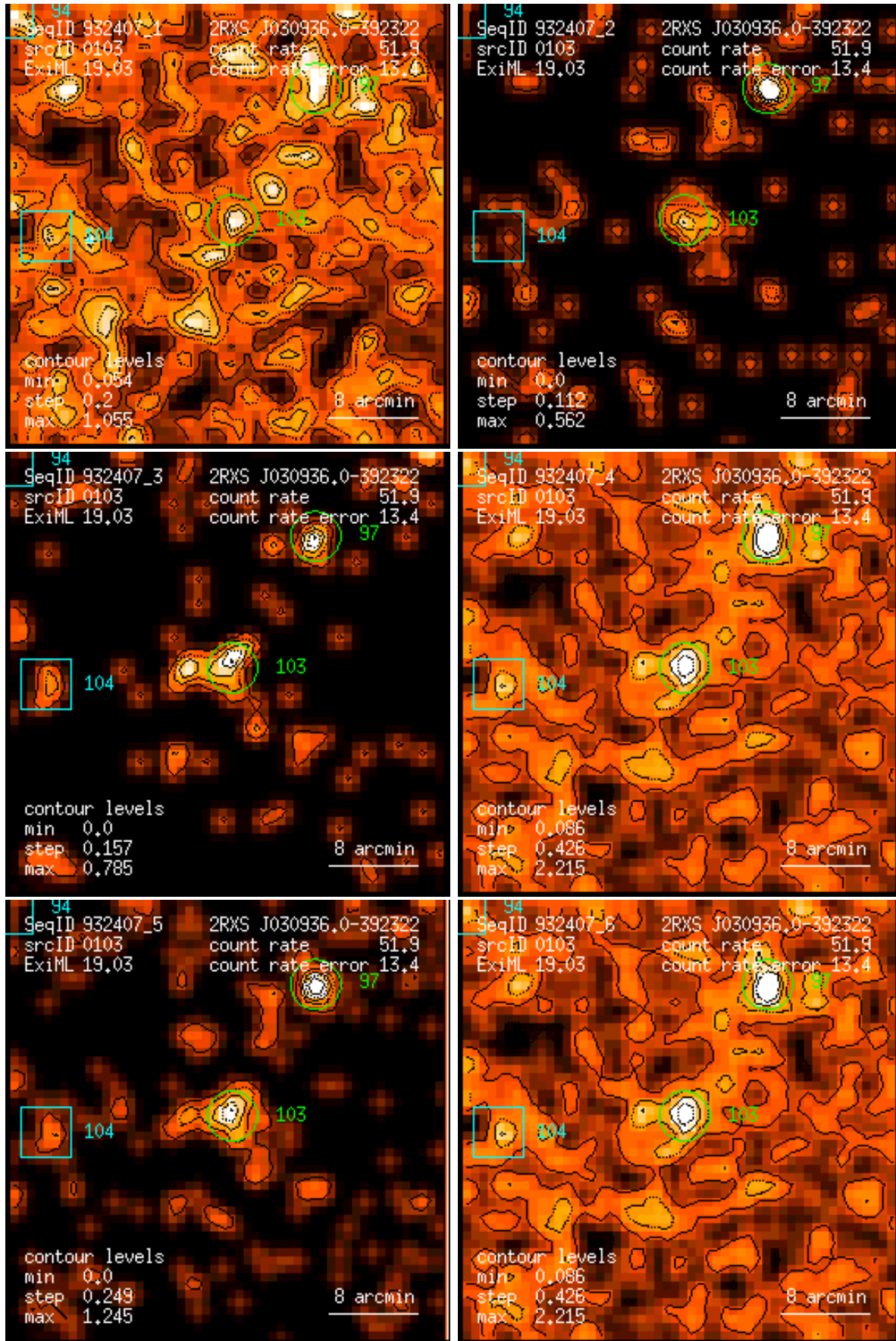
Figure 103: RASS 932407: detection 0103: band rate images, Gaussian filter: (1) PSPC channels 11 – 41, (2) 52 – 90, (3) 91 – 201, (4) 11 – 235, (5) 52 – 201, (6) 11 – 201. Broad band rates in counts/ks. Band rate contour levels in counts/ks/arcmin 2 .
