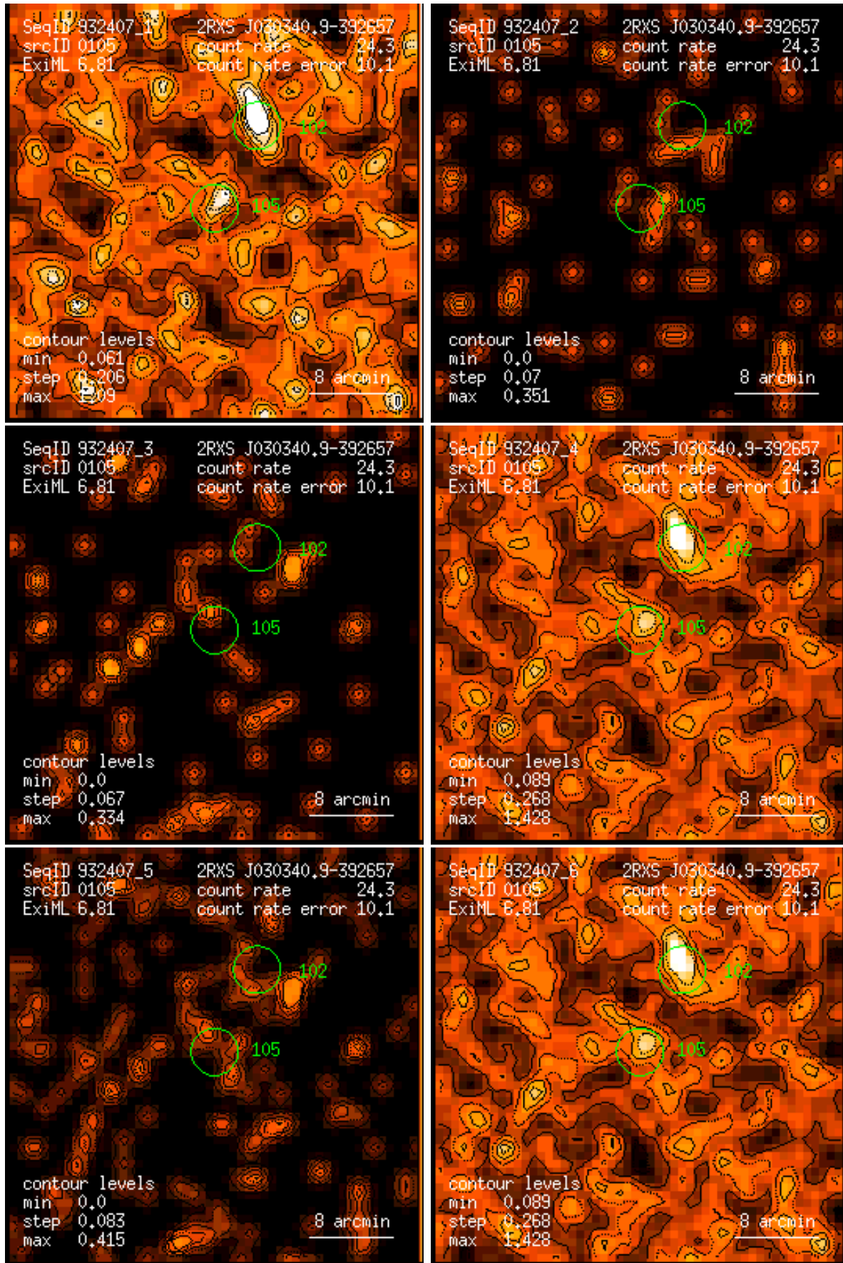
Figure 105: RASS 932407: detection 0105: band rate images, Gaussian filter: (1) PSPC channels 11 – 41, (2) 52 – 90, (3) 91 – 201, (4) 11 – 235, (5) 52 – 201, (6) 11 – 201. Broad band rates in counts/ks. Band rate contour levels in counts/ks/arcmin 2 .
