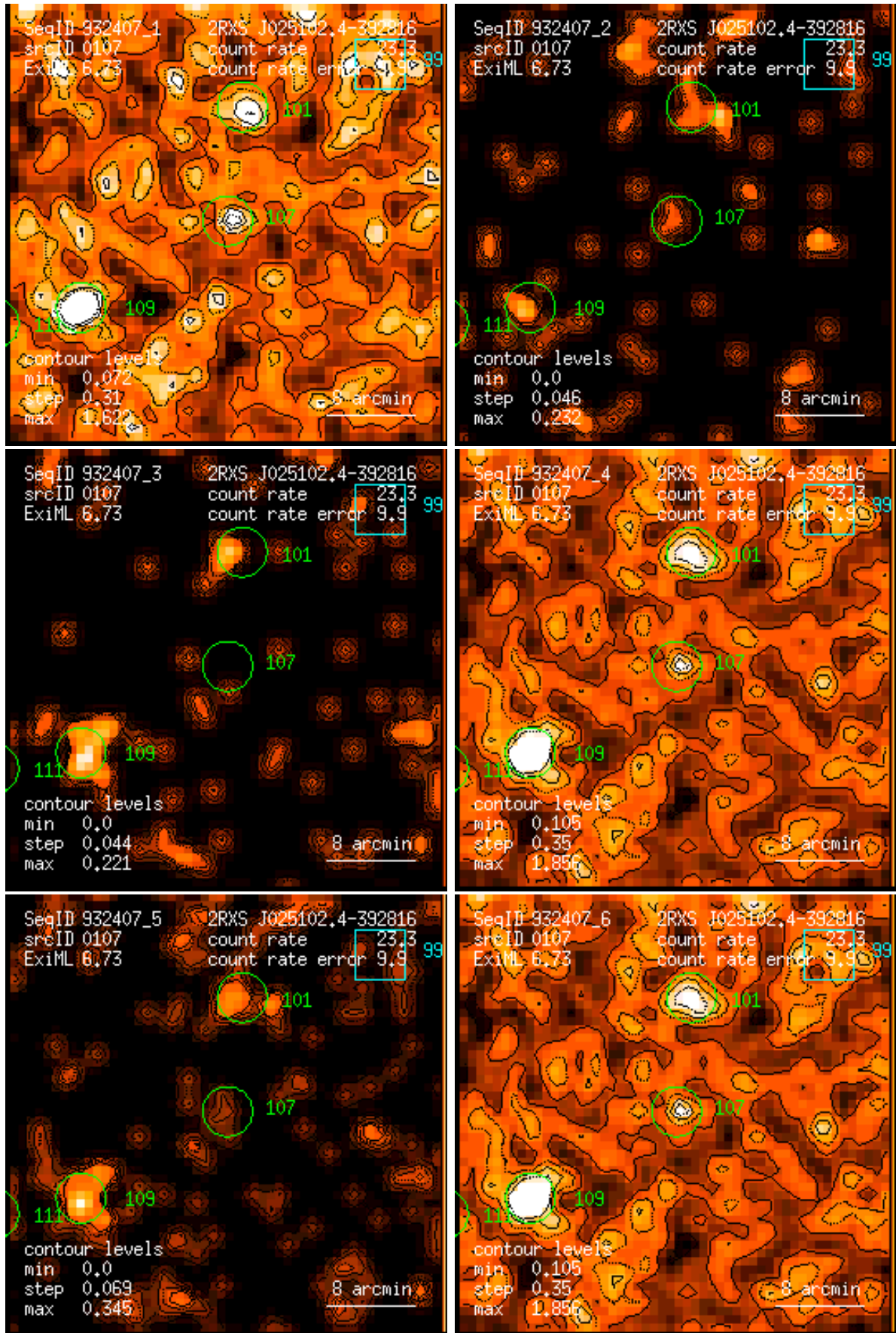
Figure 107: RASS 932407: detection 0107: band rate images, Gaussian filter: (1) PSPC channels 11 – 41, (2) 52 – 90, (3) 91 – 201, (4) 11 – 235, (5) 52 – 201, (6) 11 – 201. Broad band rates in counts/ks. Band rate contour levels in counts/ks/arcmin 2 .
