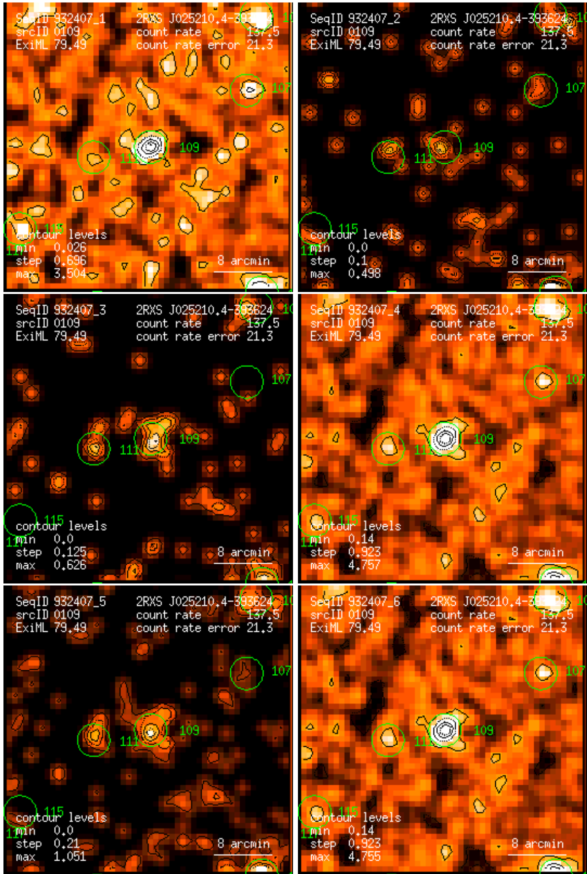
Figure 109: RASS 932407: detection 0109: band rate images, Gaussian filter: (1) PSPC channels 11 – 41, (2) 52 – 90, (3) 91 – 201, (4) 11 – 235, (5) 52 – 201, (6) 11 – 201. Broad band rates in counts/ks. Band rate contour levels in counts/ks/arcmin 2 .
