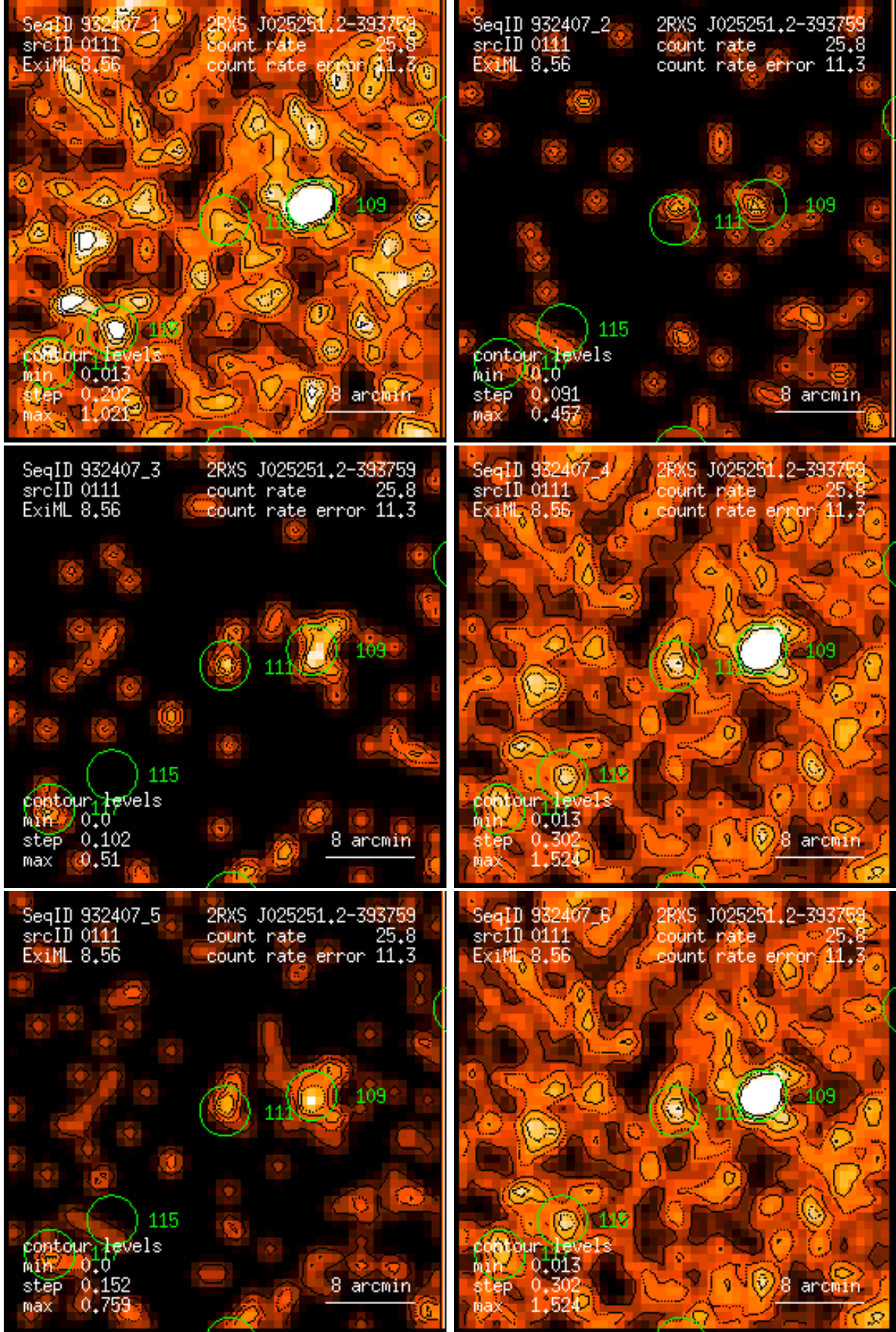
Figure 111: RASS 932407: detection 0111: band rate images, Gaussian filter: (1) PSPC channels 11 – 41, (2) 52 – 90, (3) 91 – 201, (4) 11 – 235, (5) 52 – 201, (6) 11 – 201. Broad band rates in counts/ks. Band rate contour levels in counts/ks/arcmin 2 .
